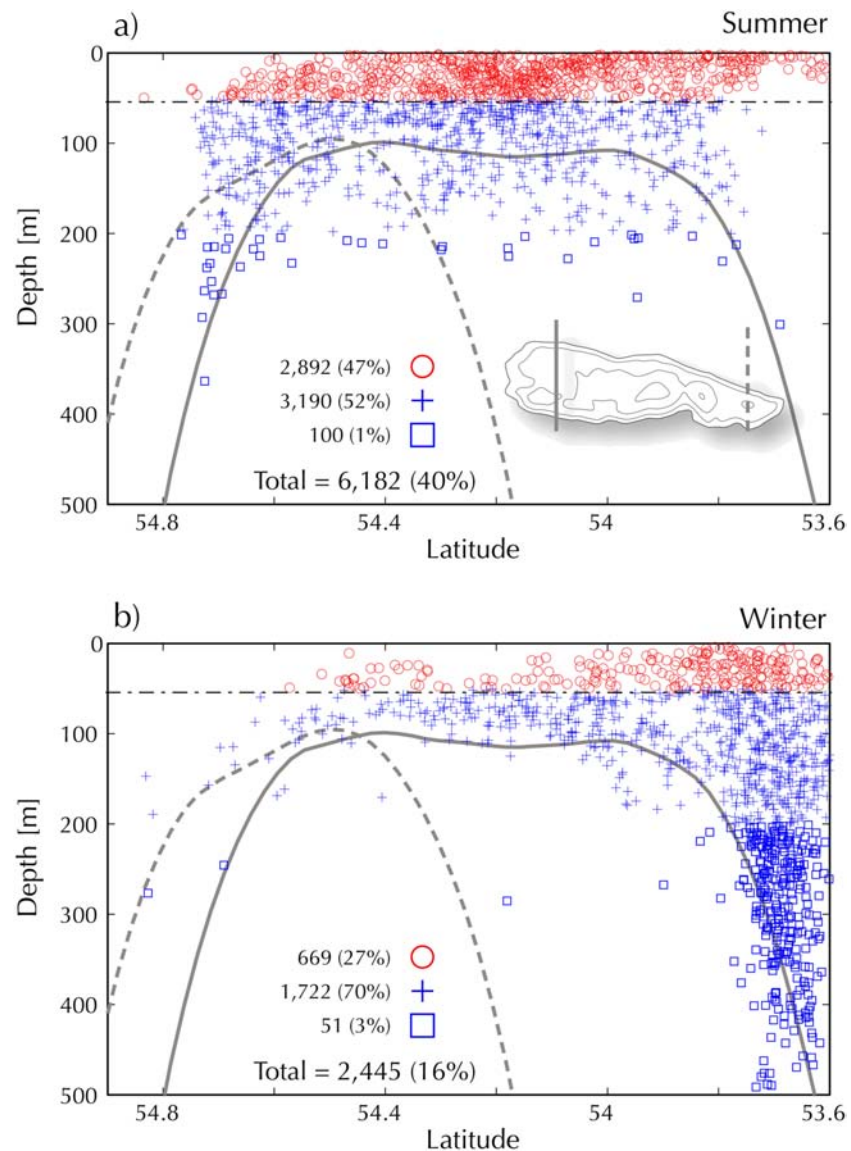
Figure 11. Floats Scattering. Meridional cross-sections showing the positions of floats released in the surface layer ( h < 50\text{ m} depth). Sampling was done after 60 days of numerical simulation. Red circles represents floats that remained above 50 m, blue crosses those that moved downward (50 to 200 m), and blue squares floats that moved below 200 m. The inset of panel (a) shows the locations of the two cross-sections.
