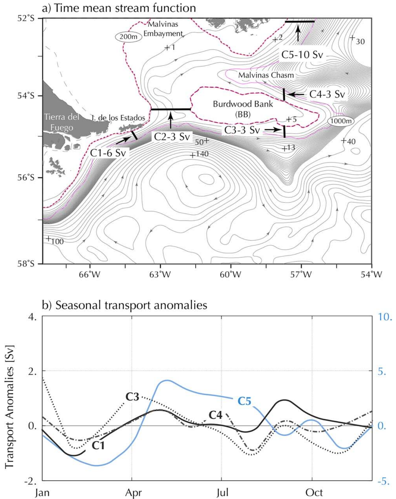
Figure 2. CTRL stream function. Top panel shows the time mean stream function of CTRL; contours are in Sverdrups ( 1 \text{ Sv} = 10^6 \text{ m}^3/\text{s} ) Red contours in top panel mark the 200- and 1,000-m isobaths. Bottom panel shows the seasonal anomalies of the volume transport through the different cross sections marked in the top panel. Anomalies are defined as the climatological monthly value minus the time mean.
