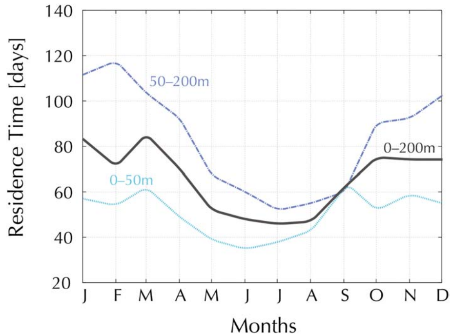
Figure 10. Residence Times. These are defined as the time it takes to evacuate 63% of the floats ( e -folding time) from the BB summit ( h < 200 m). Release depths: 0–50 m (light blue dotted line), 50–200 m (dark blue dash-dotted line), and 0–200 m (continuous black line).
