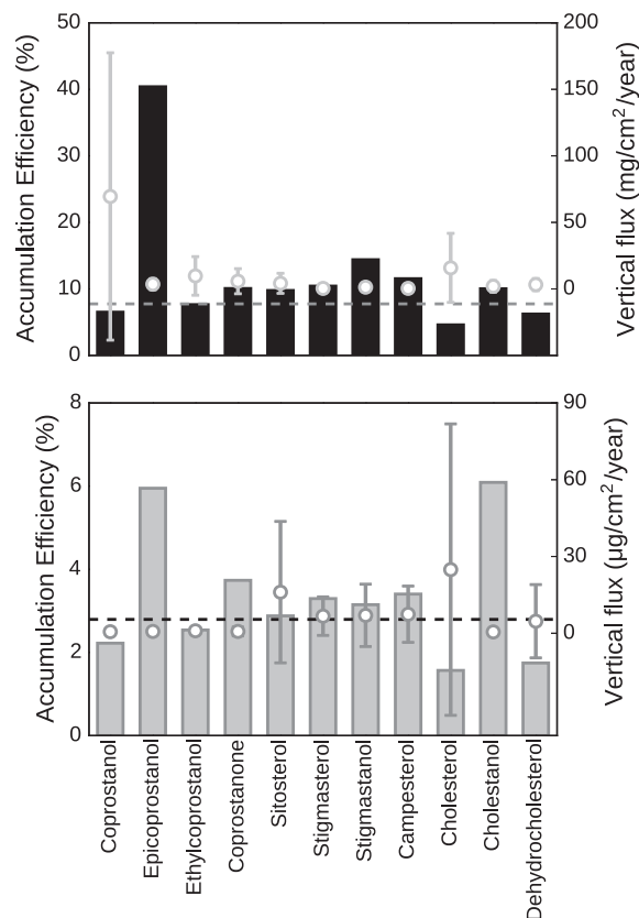
Fig. 7. Accumulation efficiencies of sterols from settling material in superficial sediments (%; bars, left axis) and vertical fluxes (points with standard error bars, right axis) for Buenos Aires (upper panel) and North (bottom panel). Horizontal dotted lines indicate accumulation efficiency of total sterols. Minor sterols ( < 1\% of total sterols) were excluded from the calculations.
