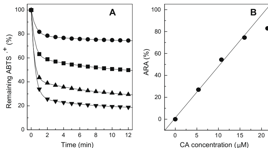
Fig. 3. (A) Kinetic behaviour of ABTS \cdot^+ for different CA concentrations. References: ● 5.37 \mu M, ■ 10.7 \mu M; ▲ 16.0 \mu M; ▼ 21.4 \mu M. (B) Linear relationship between antiradical activity percentage (ARA%) and CA concentrations.
