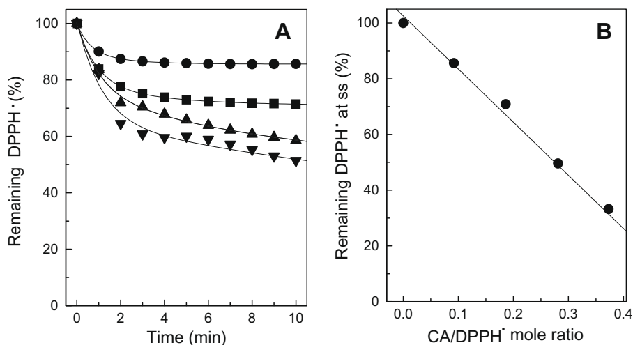
Fig. 2. (A) Kinetic profiles of DPPH \cdot consumption by CA additions. References: ● 7.3, ■ 14.5, ▲ 21.6, ▼ 28.5 \mu M of CA final concentrations. (B) Radical disappearance as a function of CA/DPPH \cdot mole ratio.
