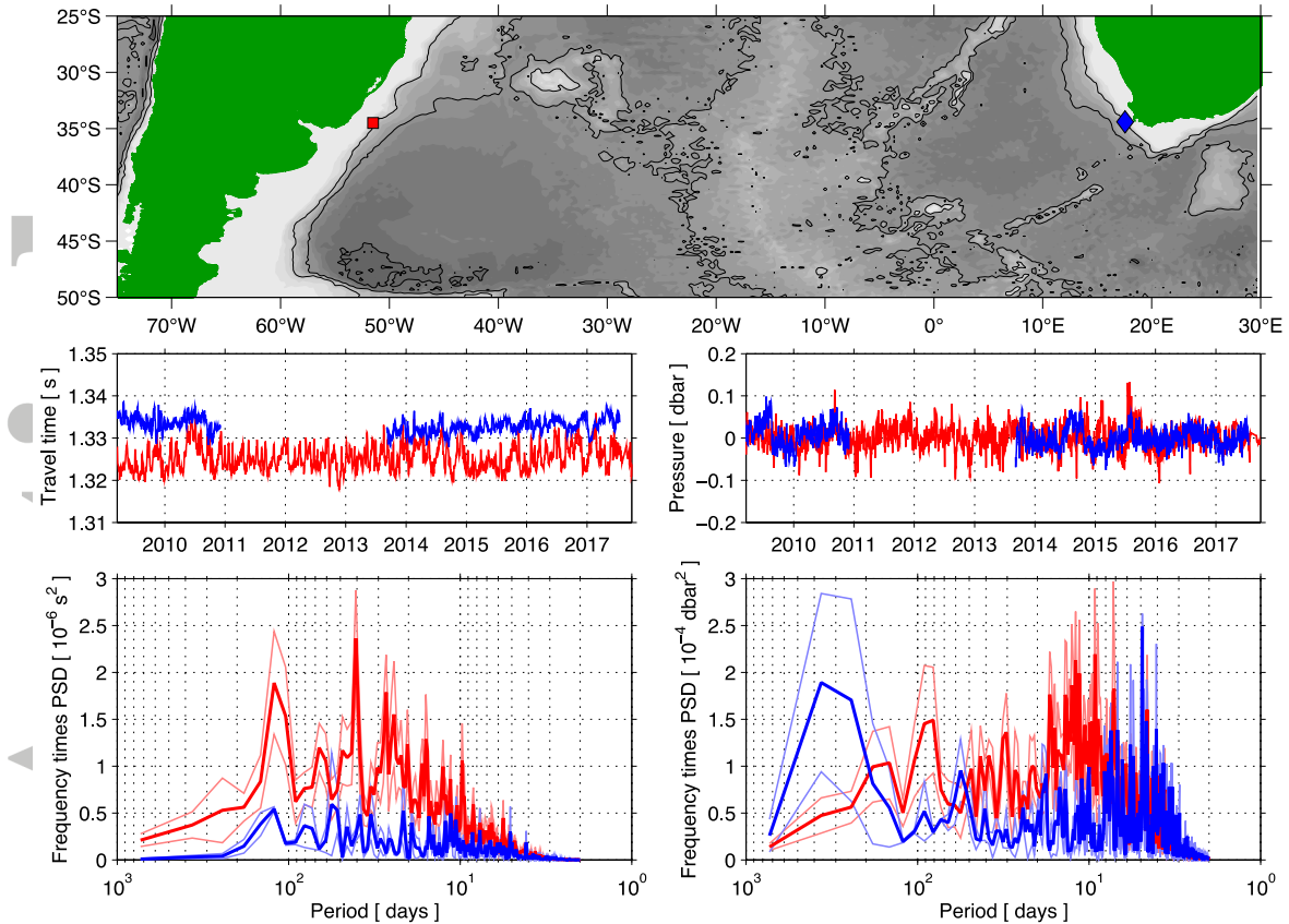
Figure 1: (a) Map showing the two moored instrument locations, Site A in the west (red) and Site Z in the east (blue), both located close to the 1350 dbar isobath; (b) daily measured round-trip acoustic travel time records, calibrated to an effective pressure level of 1000 dbar, at the western (red) and eastern (blue) sites; (c) daily measured bottom pressure records at the western (red) and eastern (blue) sites; (d) variance preserving spectra of the travel time records at the western (red) and eastern (blue) sites; (e) variance preserving spectra of the bottom pressure records at the western (red) and eastern (blue) sites. Note that the spectra for the Site Z data were computed using the continuous ~4-year records available from 2013-2017. Spectra were determined via the Welch's averaged periodogram method using a 2-year window allowing 1-year of overlap; thin lines in spectra indicate 67% confidence limits. Topography in the top panel (gray shading with 500 m intervals; every 2000 m contour shown as black contour) is from Smith and Sandwell (1997).
