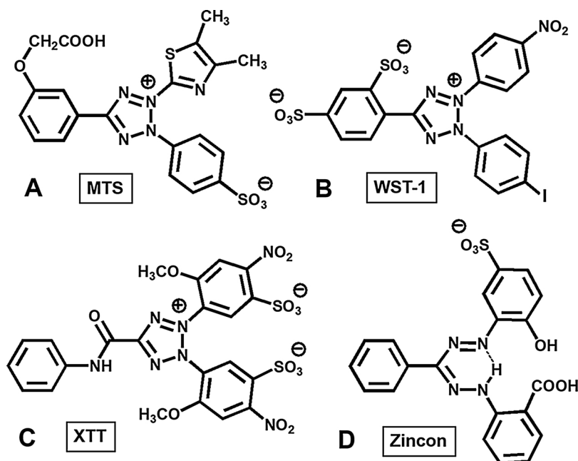
Fig. 2. Examples of sulfonated derivatives of tetrazolium salts and a formazan reagent. A: MTS. B: WST-1. C: XTT. D: Zincon.
