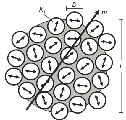
Fig. 8. Random anisotropy model for nanocrystalline materials. Double arrows indicate the randomly oriented anisotropy ( K_1 is the first-order anisotropy constant) within the structural correlation length (grain size, D ). The long arrow indicates the orientation of the magnetization ( \mathbf{m} ) within the magnetic correlation length ( L ). [Reproduced from (53)]
