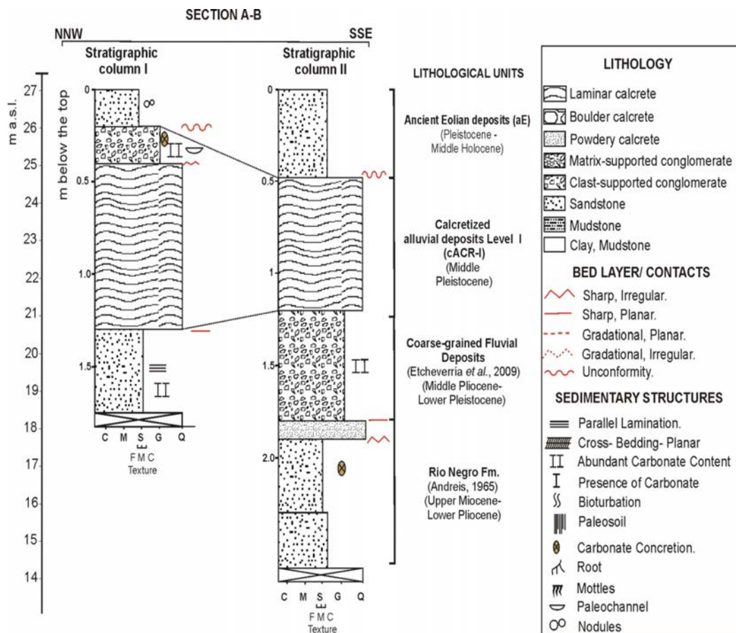
FIG. 4. Section A-B representing the integration of the stratigraphic columns I and II oriented in a NNW to SSE transect (see Fig. 2). The stratigraphic columns I and II are located according to their altitudinal position. The vertical scale has been exaggerated with respect to the altitudinal scale.
