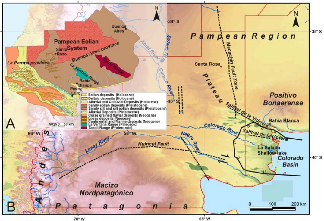
FIG. 1. A. Regional geological map (modified after Lizuáin et al. , 1998); B. Structural sketch map showing the main faults in the study area and the Colorado Basin (modified after Vogt et al. , 2010).
