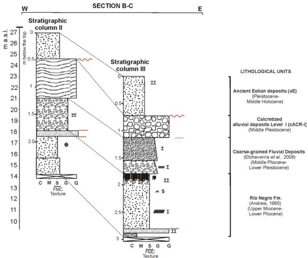
FIG. 6. Section B-C representing the integration of the stratigraphic columns II and III oriented in a W-E transect (see Fig. 2). The stratigraphic columns II and III are located according to their altitudinal position. The vertical scale has been exaggerated with respect to the altitudinal scale.
