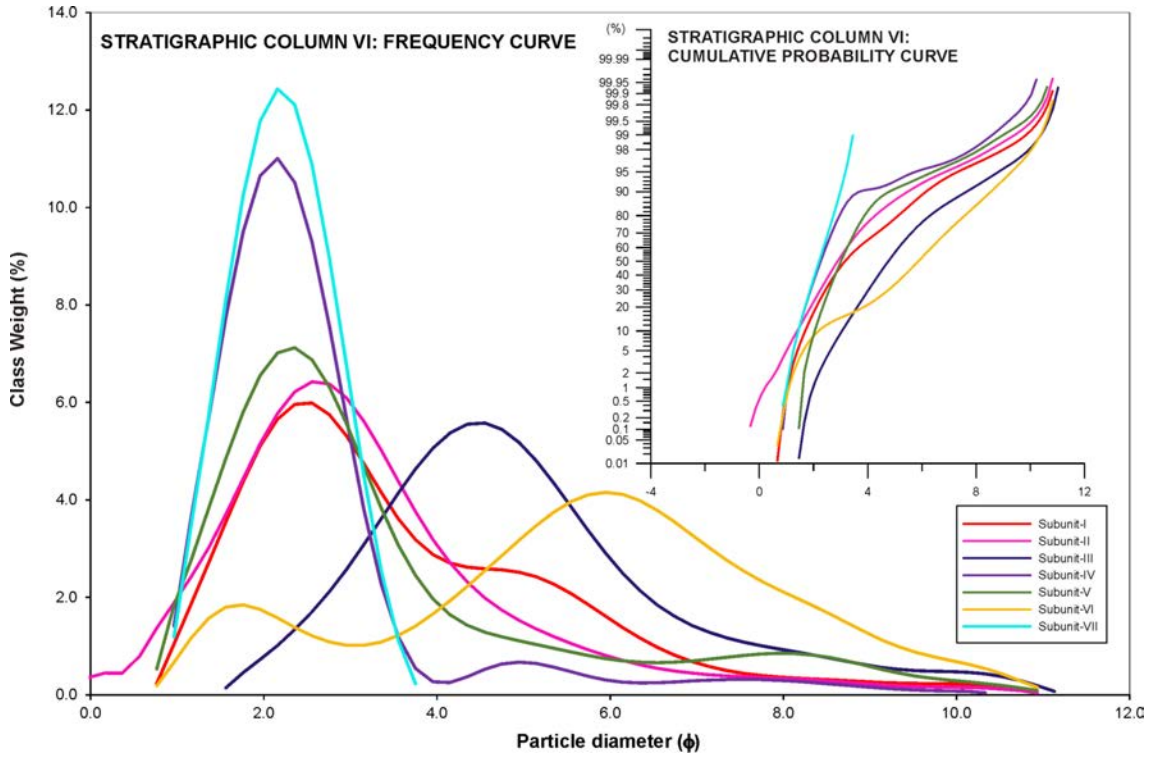
FIG. 2. Frequency and cumulative probability curves of each subunit identified in the stratigraphic column VI. The cumulative probability curves according to (Mycielska-Dowgiało and Ludwikowska-Kędzia, 2011) are first group for all the subunit except for the subunits IV, which indicate an eolian and fluvial-eolian origin respectively. The frequency curves show a unimodal distribution for all subunits except for the subunit IV.
