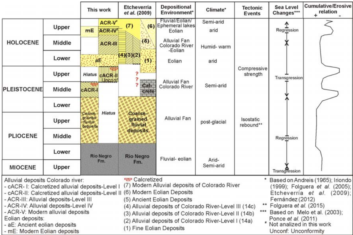
FIG. 10. Integrated stratigraphic column of the lithological units observed in this work and their environmental interpretation. Also, the figure shows the correlation with the units defined by Etcheverría et al. (2009) in the area.
