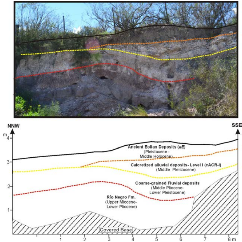
FIG. 5. Exposed section in the stratigraphic columns II locality. It is localized to the West of the La Salada shallow lake oriented NNW to SSE. It exposes the folding of the Miocene-Pleistocene units and the sharp erosive contact on which overlies aE deposits.
