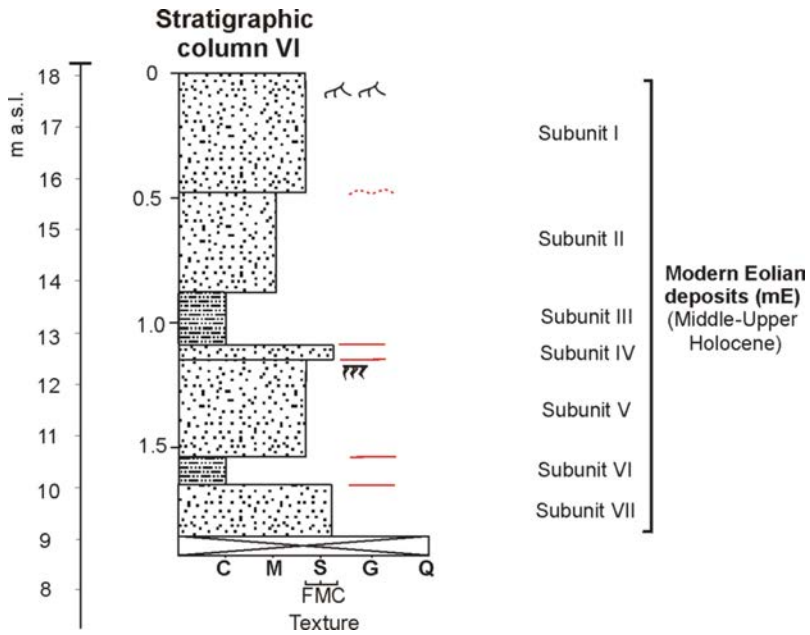
FIG. 9. The stratigraphic columns VI located west of La Salada shallow lake (see Fig. 2). The vertical scale has been exaggerated with respect to the altitudinal scale. This is localized at 18 m a.s.l. The deposits of the stratigraphic column VI overlies the Río Negro Formation. This is suggested by an outcrop of Río Negro Formation in the shoreline of La Salada.
