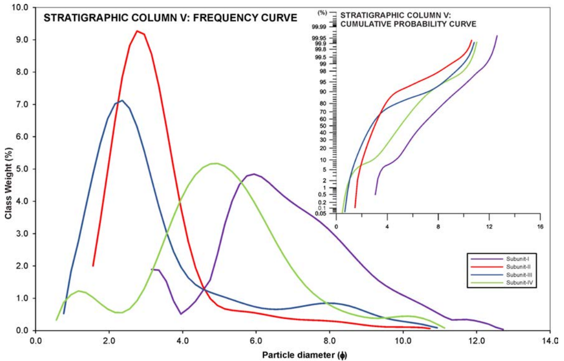
FIG. 1. Frequency and cumulative probability curves of each subunits in the stratigraphic column V. The cumulative probability curves according to (Mycielska-Dowgiało and Ludwikowska-Kędzia, 2011) are third group for the subunits I and IV and the first group for subunits II and III, which indicate a Fluvial-eolian and eolian origin respectively. The frequency curves show a bimodal distribution for the subunits I and IV while for the subunits II and III are unimodal.
