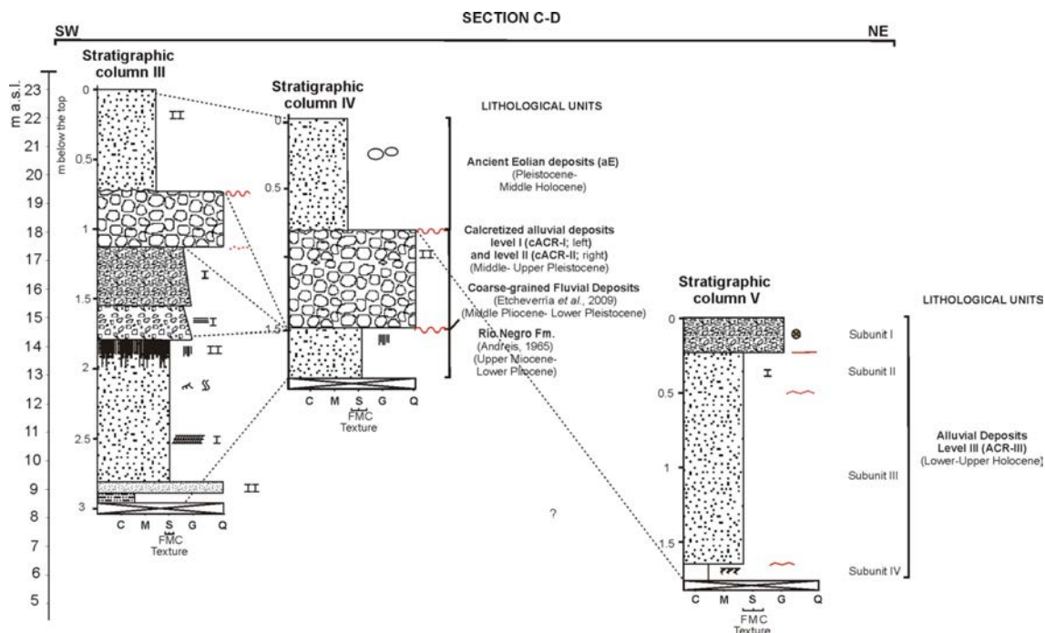
FIG. 8. Section C-D representing the integration of the stratigraphic columns III, IV and V oriented in SW-NE transect (see Fig. 2). The stratigraphic columns III, IV and V are located according to their altitudinal position. The vertical scale has been exaggerated with respect to the altitudinal scale. Observe the topographic difference among the stratigraphic columns III, IV and V, localized at 23, 22 and 15 m a.s.l. respectively, which are associated to three different terrace levels.
