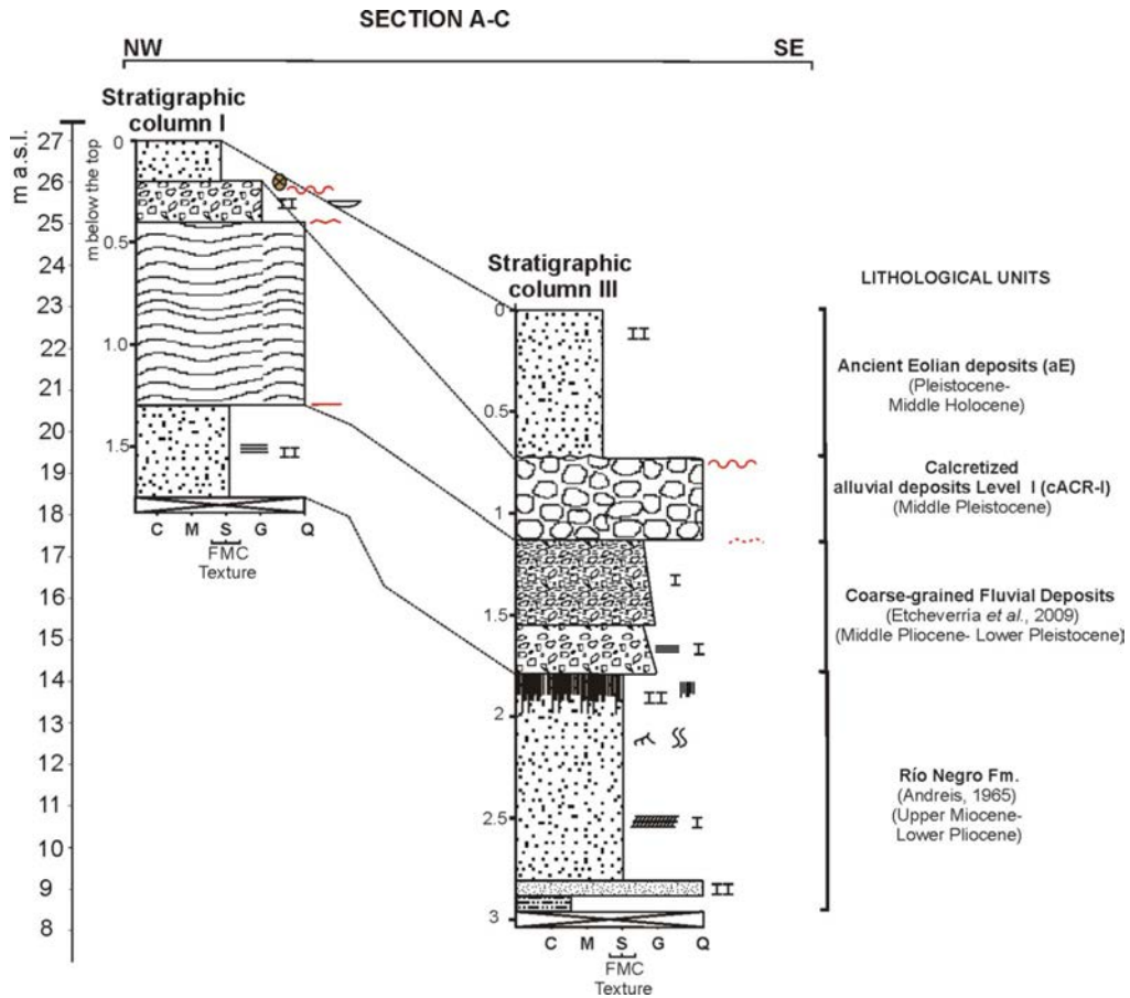
FIG. 7. Section A-C representing the integration of the stratigraphic columns I and III oriented in NW- SE transect (see Fig. 2). The stratigraphic columns I and III are located according to their altitudinal position. The vertical scale has been exaggerated with respect to the altitudinal scale. Observe the topographic difference among the stratigraphic columns I and III, localized at 27, and 23 m a.s.l. respectively.
