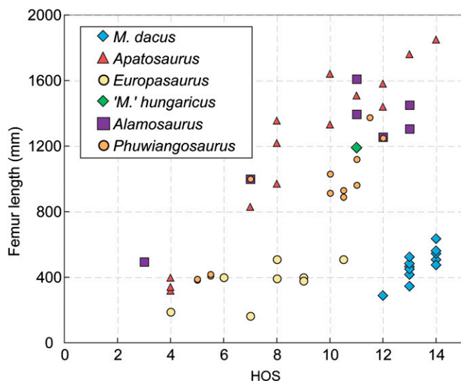
Fig. 3. Plot of histologic ontogenetic stage (HOS) (35) vs. body size as expressed by femur length in Magyarosaurus dacus , compared with Europasaurus , Apatosaurus , Alamosaurus , and Phuwiangosaurus . The samples of Magyarosaurus dacus derive from humeri that were normalized to femur length. The single " M. " hungaricus sample is also included. Data for Alamosaurus were obtained from a previous report (38), supported by own data. Data for Phuwiangosaurus were obtained from another report (37).
