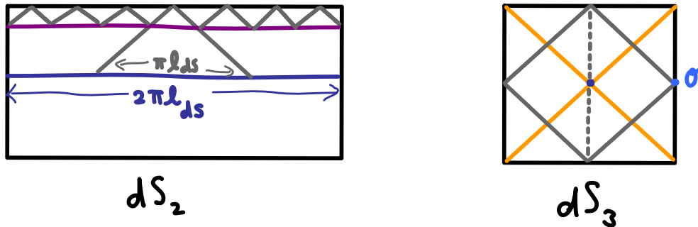
Figure 4. The left panel contains the dS_2 Penrose diagram; the vertical sides are identified. The dark blue line at \tau = 0 corresponds to the central dot (a circle of radius \ell_{dS} ) in the dS_3 diagram from figure 2, reproduced here on the right. This full circle of size 2\pi\ell_{dS} is the horizon for the observer \mathcal{O} on the far right, causally connected to it through the dS_3 bulk. Within the global dS_2 geometry, the segments with extremal area \pi\ell_{dS} between the end points are the largest for which the endpoints can communicate, as derived in the text. On a late-time slice, indicated in purple, we show a string of causal segments whose extremal area is \pi\ell_{dS} and entanglement entropy is \pi c/6 .
