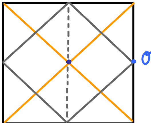
Figure 2. The Penrose diagram of dS_{d+1} , with the UV slice w = \pi \ell_{\text{dS}}/2 of the geometry indicated by the dashed grey line. The solid grey lines indicate the two deep IR regions, w = 0 and w = \pi \ell_{\text{dS}} . The RT surface S^{d-1} is in the center of the diagram, indicated as a dark blue point. Its area determines the entanglement entropy between the two matter sectors. and tracing out the second sector gives a maximally mixed density matrix \rho_1 for the first. It is also the Gibbons-Hawking horizon entropy for an observer momentarily at the deep IR end of the second warped throat at \tau = 0 , indicated in light blue. That observer has no interaction with the first matter sector and must trace it out.
