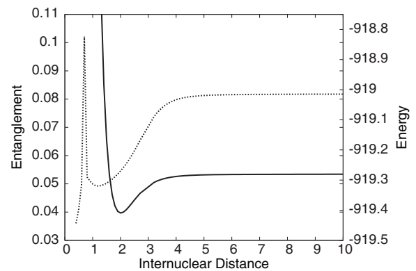
Figure 13. Entanglement (solid line) and total energy (dotted line) for the dissociation process of the chlorine molecule.
