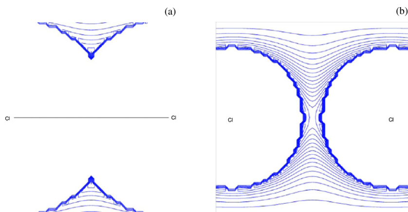
Figure 16. Contours of the isosurface of the MEP for the dissociation process of the chlorine molecule at an internuclear distance of 2.2 Å (left) and 3.0 Å (right).
