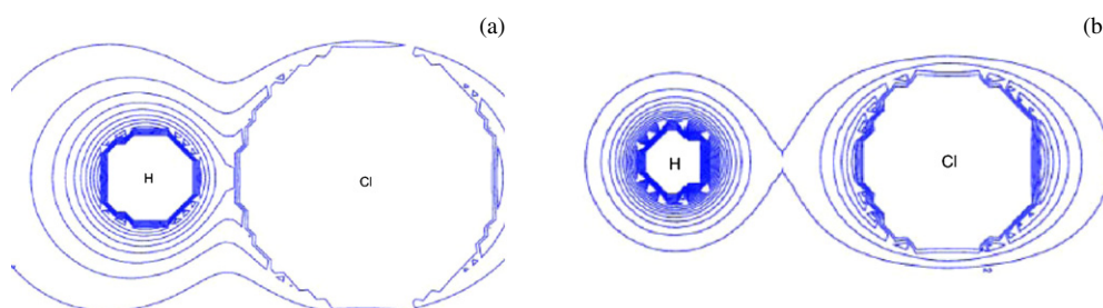
Figure 20. Contours of the isosurface of the MEP for the dissociation process of the hydrogen chloride molecule at an internuclear distance of 2.0 Å (left), and 3.6 Å (right).
