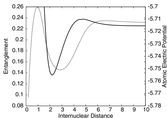
Figure 10. Entanglement (dotted line) and atomic EP (solid line) for the dissociation process of the lithium molecule.
