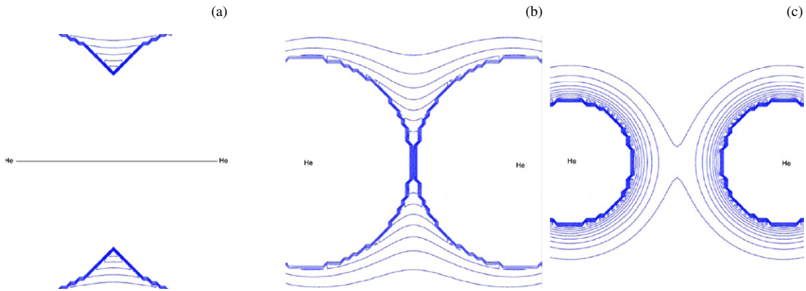
Figure 8. Contours of the isosurface of the MEP for the dissociation process of the helium excimer at an internuclear distance of 1.2 Å (left), 1.6 Å (center) and 2.6 Å (right).
