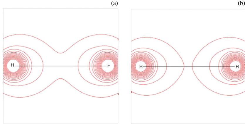
Figure 3. Contours of the isosurface of the LAP for the dissociation process of the hydrogen molecule at an internuclear distance of 0.72 Å (left) and 0.76 Å (right).
