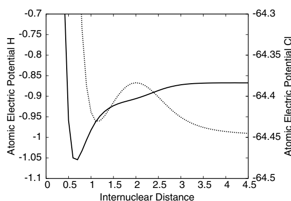
Figure 18. Atomic EP for chlorine (solid line) and hydrogen (dotted line) for the dissociation process of the hydrogen chloride molecule.
