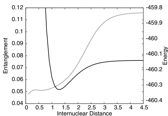
Figure 17. Entanglement (dotted line) and total energy (solid line) for the dissociation process of the hydrogen chloride molecule.
