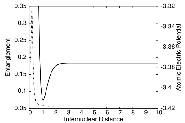
Figure 6. Entanglement (dotted line) and the atomic EP (solid line) for the dissociation process of the helium excimer.
