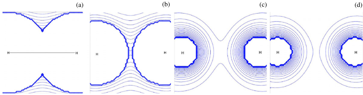
Figure 4. Contours of the isosurface of the MEP for the dissociation process of the hydrogen molecule at an internuclear distance of 0.78 Å (left), 1.0 Å, 2.2 Å and 2.5 Å (right).
