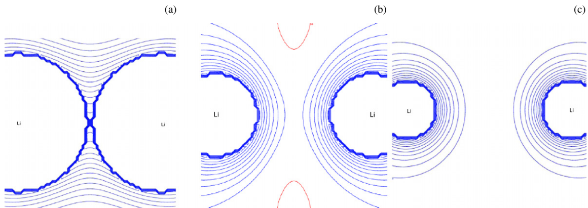
Figure 12. Contours of the isosurface of the MEP for the dissociation process of the lithium molecule at an internuclear distance of 2.1 Å (left), 3.6 Å (center) and 5.5 Å (right).
