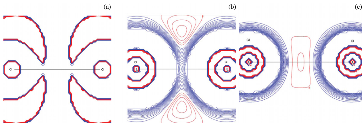
Figure 15. Contours of the isosurface of the LAP for the dissociation process of the chlorine molecule at an internuclear distance of 0.8 Å (left), 1.2 Å (center) and 1.9 Å (right).
