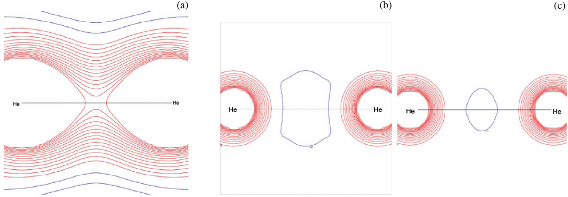
Figure 7. Contours of the isosurface of the LAP for the dissociation process of the helium excimer at an internuclear distance of 0.5 Å (left), 1.0 Å (center) and 1.05 Å (right).
