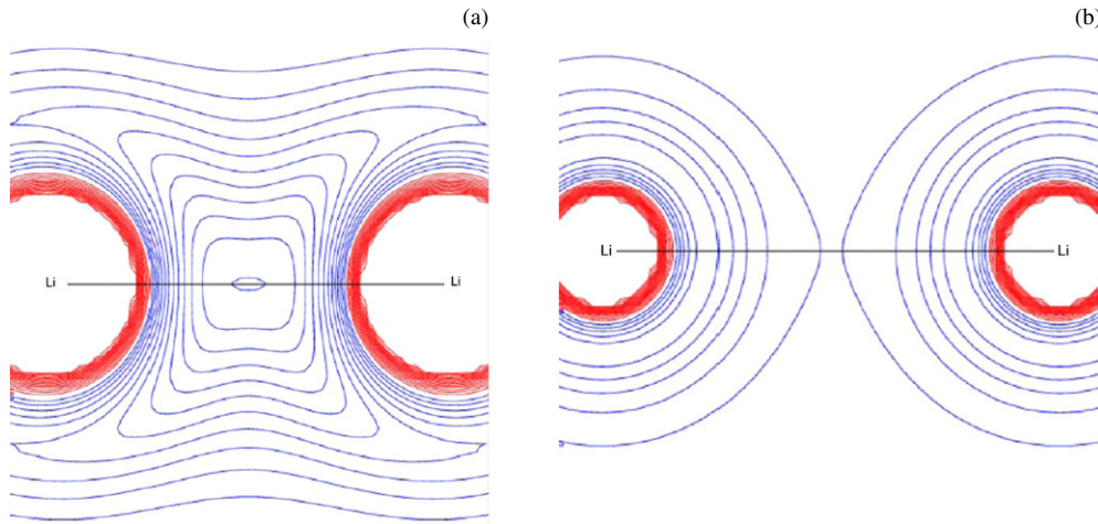
Figure 11. Contours of the isosurface of the LAP for the dissociation process of the lithium molecule at an internuclear distance of 0.9 Å (left) and 1.4 Å (right).
