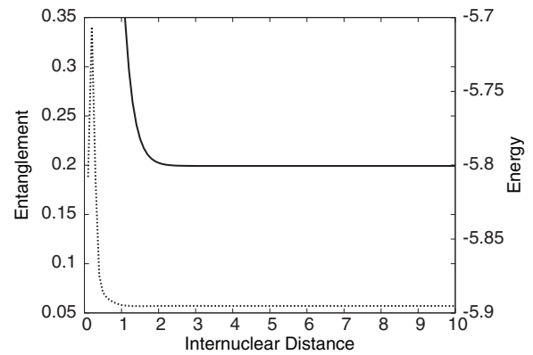
Figure 5. Entanglement (dotted line) and total energy (solid line) for the dissociation process of the excimer of helium.
