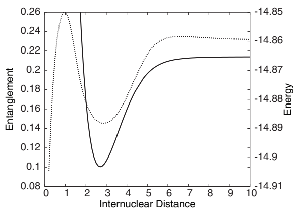
Figure 9. Entanglement (dotted line) and total energy (solid line) for the dissociation process of the lithium molecule.
