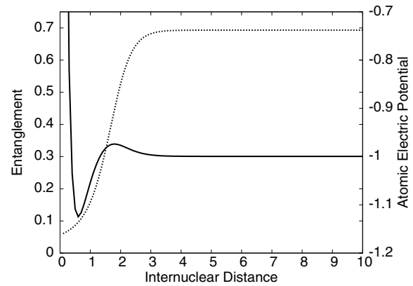
Figure 2. Entanglement (dotted line) and the atomic EP (solid line) for the dissociation process of the hydrogen molecule.
