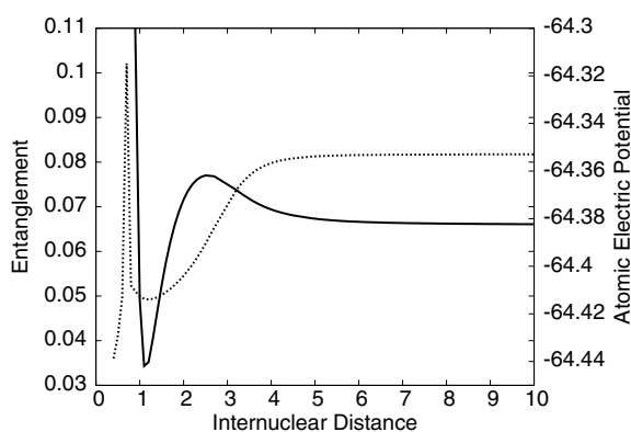
Figure 14. Entanglement (dotted line) and the atomic EP (solid line) for the dissociation process of the chlorine molecule.
