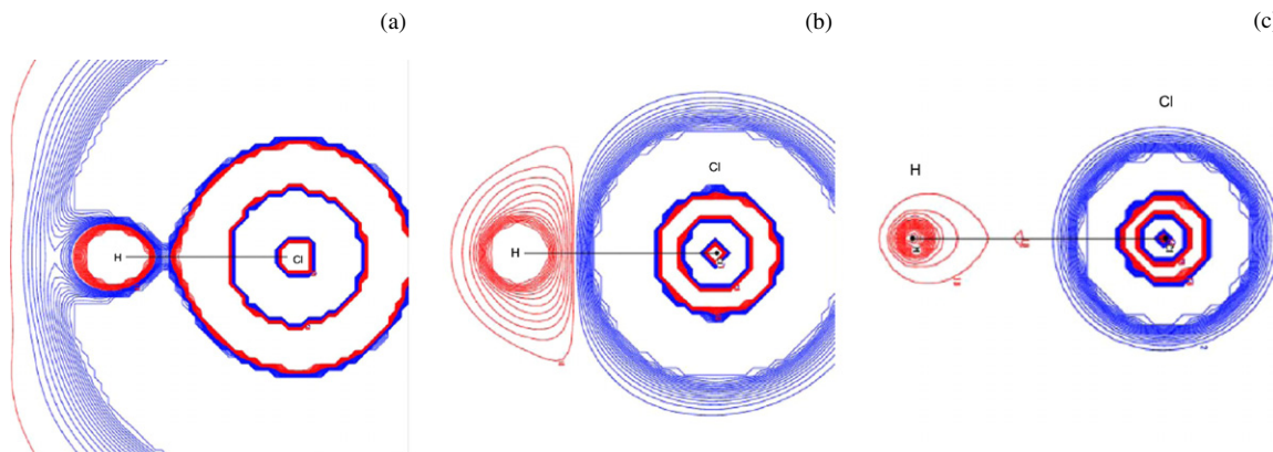
Figure 19. Contours of the isosurface of the LAP for the dissociation process of the hydrogen chloride molecule at an internuclear distance of 0.35 Å (left), 0.7 Å (center) and 1.25 Å (right).
