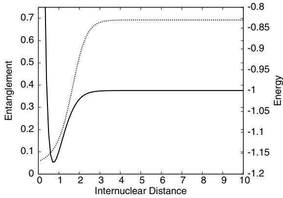
Figure 1. Entanglement (dotted line) and total energy (solid line) for the dissociation process of the hydrogen molecule.
