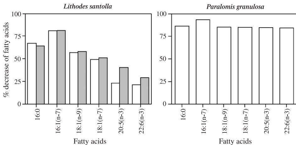
Fig. 2. L. santolla and P. granulosa . Fatty acid utilization during lecithotrophic larval development, expressed as percentage decrease of major individual fatty acids (mean data from experiments with fed and unfed larvae). Decrease was calculated from fatty acid amount of zoea after hatching (day 0) and latest megalopa analyzed (day 62 for L. santolla and day 52 for P. granulosa ) (open bars). In addition, the same calculation is presented until the juvenile stage of L. santolla (gray bars).
