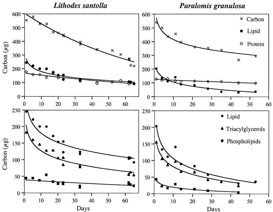
Fig. 1. L. santolla and P. granulosa . Changes in biochemical composition during lecithotrophic larval development; all data are converted to \mu\text{g} carbon (C) per larva. Carbon content with exponential fit for L. santolla ( y = 595.43e - 0.0134x ) and logarithmic fit for P. granulosa ( y = -68.038\ln(x) + 572.05 ); total lipid with logarithmic fit for L. santolla ( y = -39.967\ln(x) + 271.55 ) and P. granulosa ( y = -43.535\ln(x) + 205.85 ); protein with exponential fit for L. santolla ( y = 168.13e - 0.0091x ) and P. granulosa ( y = 124.96e - 0.0045x ); triacylglycerols with logarithmic fit for L. santolla ( y = -34.083\ln(x) + 204.92 ) and P. granulosa ( y = -32.709\ln(x) + 156.36 ); phospholipids with exponential fit for L. santolla ( y = 39.348e - 0.0081x ) and logarithmic fit for P. granulosa ( y = -9.3307\ln(x) + 41.019 ).
