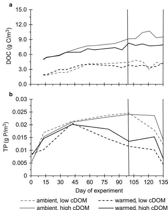
FIG. 4. Concentrations of (a) dissolved organic carbon (DOC) and (b) total phosphorus (TP) over the course of the experiment. Values shown are means over the four replicates of each treatment. Vertical lines bracket the time window (day 100–135) over which all other response variables were averaged.
