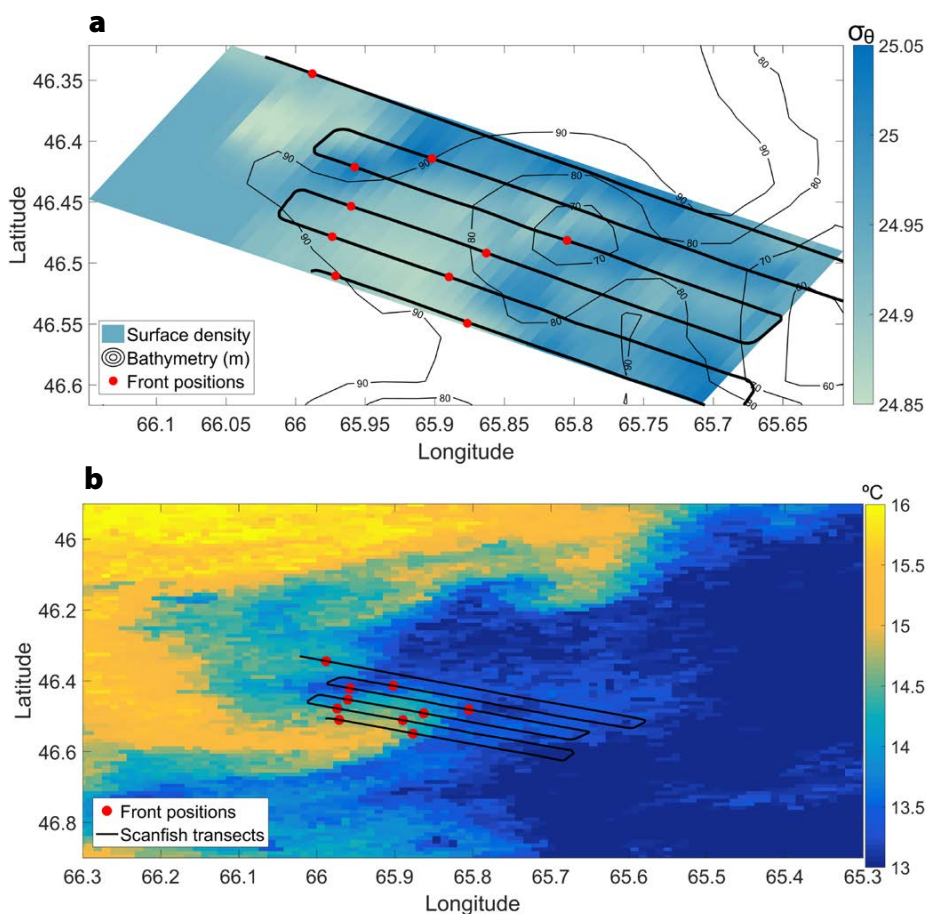
FIGURE 2. Frontal positions in the SJG during neap tide (red points). The colors represent average potential density between 3 m and 10 m depth in panel (a), and sea surface temperature ( ^{\circ}\text{C} ) derived from satellite sensors in panel (b). Data processing and figure construction were done using MATLAB (R2016a), and Gibbs Sea Water routines for MATLAB were used to treat the seawater thermodynamics data (McDougall and Barker, 2011).
