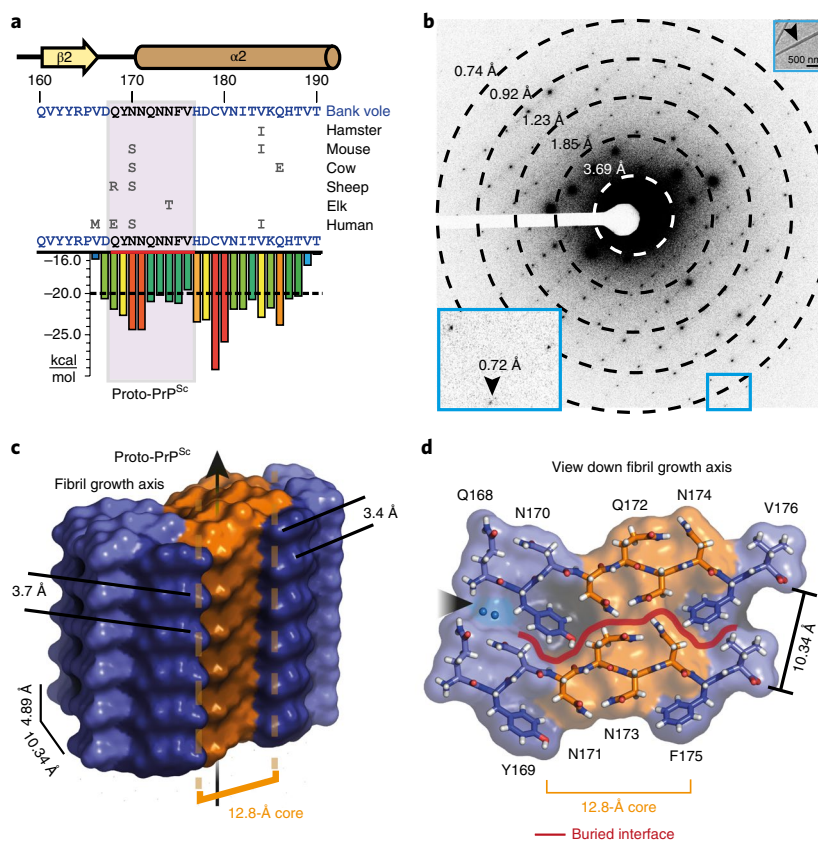
Fig. 1 | Structure of proto-PrP Sc from sub-ångström diffraction of nanoscale crystals by MicroED. a , Sequence of the bank vole PrP \beta 2- \alpha 2 loop, highlighting local secondary structure and variation in sequence compared to hamster, mouse, cow, sheep, elk, and human. The sequence of proto-PrP Sc is highlighted in a plot that indicates propensity for amyloid formation (scored in kcal/mol). The region encoding proto-PrP Sc is boxed in magenta. b , Single MicroED image showing strong diffraction to 0.72 Å (inset). A second inset shows a proto-PrP Sc crystal probed by MicroED (arrow). c,d , Side ( c ) and top ( d ) views of the proto-PrP Sc -molecular surface. Stacked aromatics are colored dark purple, a conformationally constrained core region is colored orange, two waters are noted with a black arrow, and a red line indicates the interface between sheets in d .
