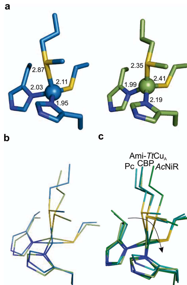
Fig. 5 Structure of the Ami- TtCu A copper site. (a) Copper sites of amicyanin (1AAC, left) and Ami- TtCu A (5U7N, right). (b) Overlay of the Cu sites of amicyanin (1AAC, blue) and Ami- TtCu A (5U7N, green). Note that the Ami- TtCu A site adopts a slightly tetragonally distorted conformation with the copper atom displaced from the N–S–N plane. (c) Coupled distortion model exemplified by an overlay of the active sites of plastocyanin (1PLC), cucumber basic protein (2CBP), Ami- TtCu A (5U7N) and nitrite reductase (1NIF). The arrow indicates the direction of the distortion.
