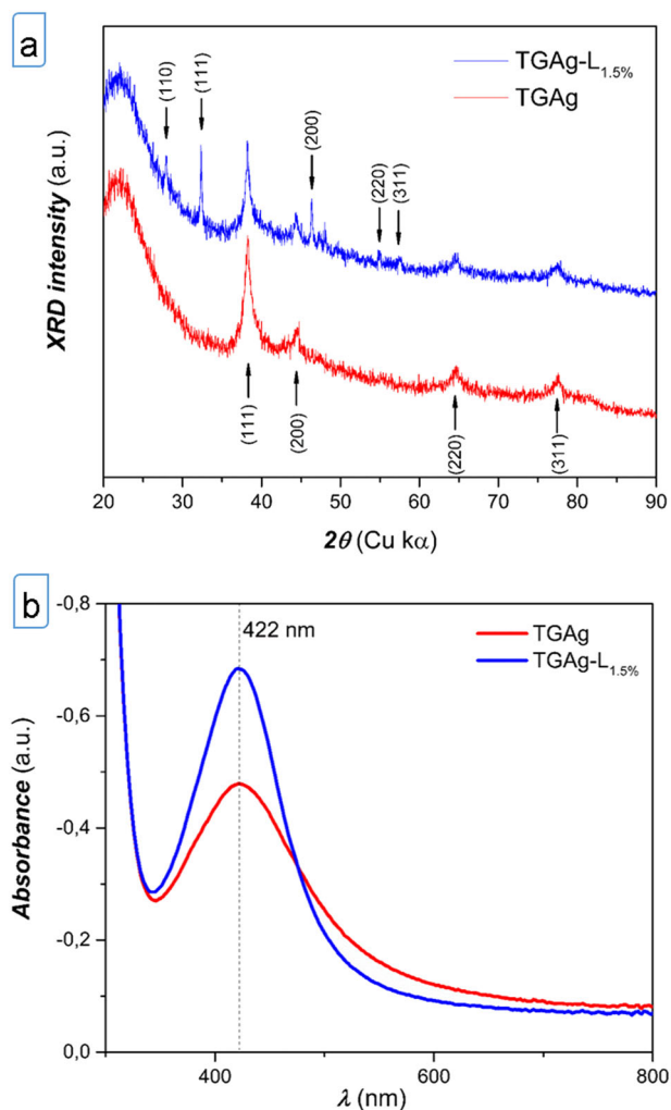
Fig. 6 a XRD and b UV-visible spectra of TGAg and TGAg-L 1.5% samples thermally densified at 150 °C
