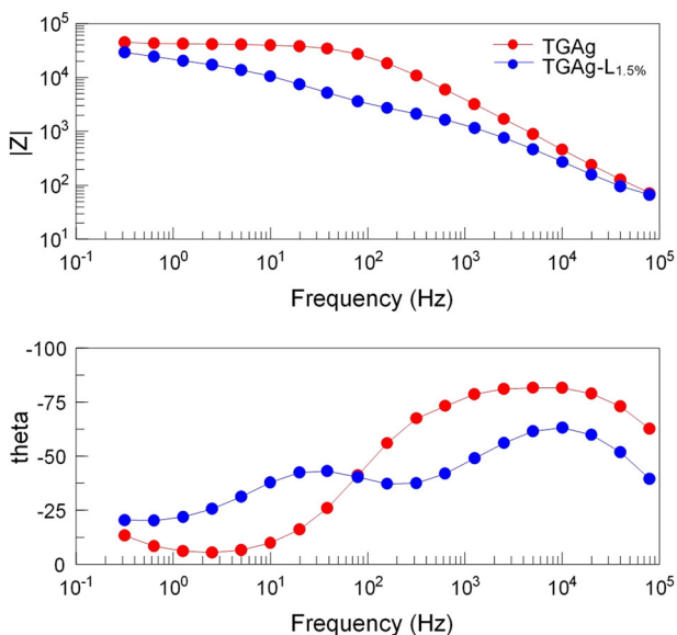
Fig. 8 Bode representation for TGAg (red dots) and TGAg-L 1.5% (blue dots) coatings exposed at 0.01 mol L -1 NaCl aerated solution
