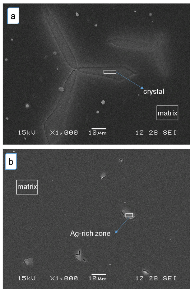
Fig. 4 a SEM micrograph of crystal formation on TGAg coating stored 7 days at RT without thermal treatment and b SEM micrograph of TGAg-L 1.5% coating stored 7 days at RT displaying Ag-rich zones
