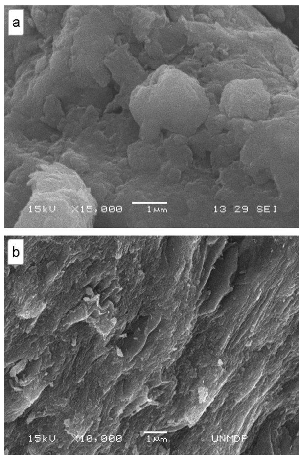
Fig. 1 Scanning electron microscopy of Laponite® S482 (a) as-received and (b) stratified after its exfoliation in water and a reprecipitation process
