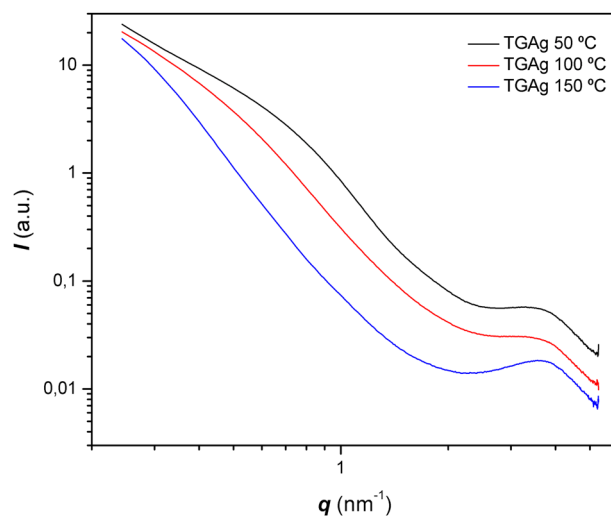
Fig. 2 SAXS curves of TGAg coatings treated at different temperatures
