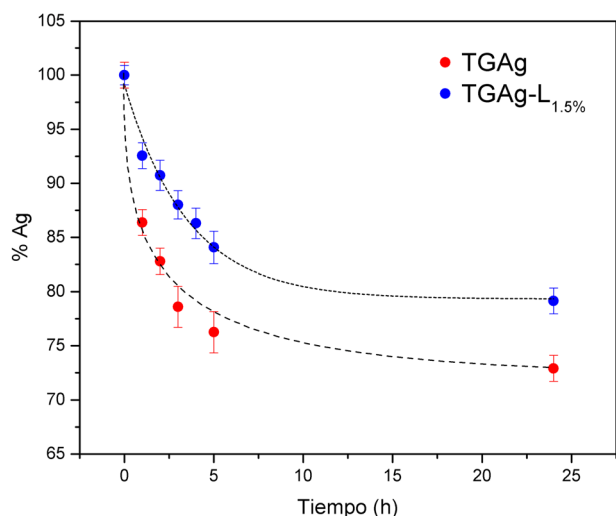
Fig. 9 Curves of silver releasing for TGAg (red dots) and TGAg-L 1.5% (blue dots) samples, subjected to a lixiviation process to different times
