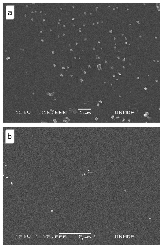
Fig. 5 Scanning Electron Microscopy of (a) TGAg and (b) TGAg-L 1.5% surfaces thermally densified at 150 °C
