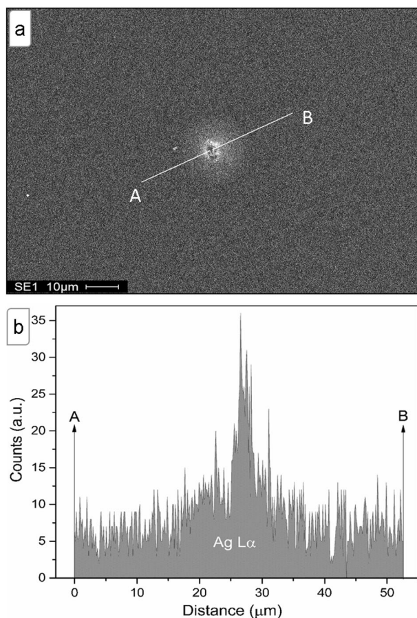
Fig. 7 a SEM image of a TGAg surface particle and EDAX line scan microanalysis, the white line is the pathway where EDS analysis was performed, and b Ag L- \alpha line profile in the scan microanalysis
