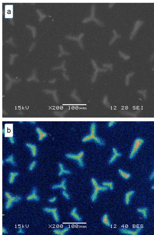
Fig. 3 a SEM micrograph of TGAg coating stored at RT, without thermal treatment, and b image obtained from backscattered electrons
