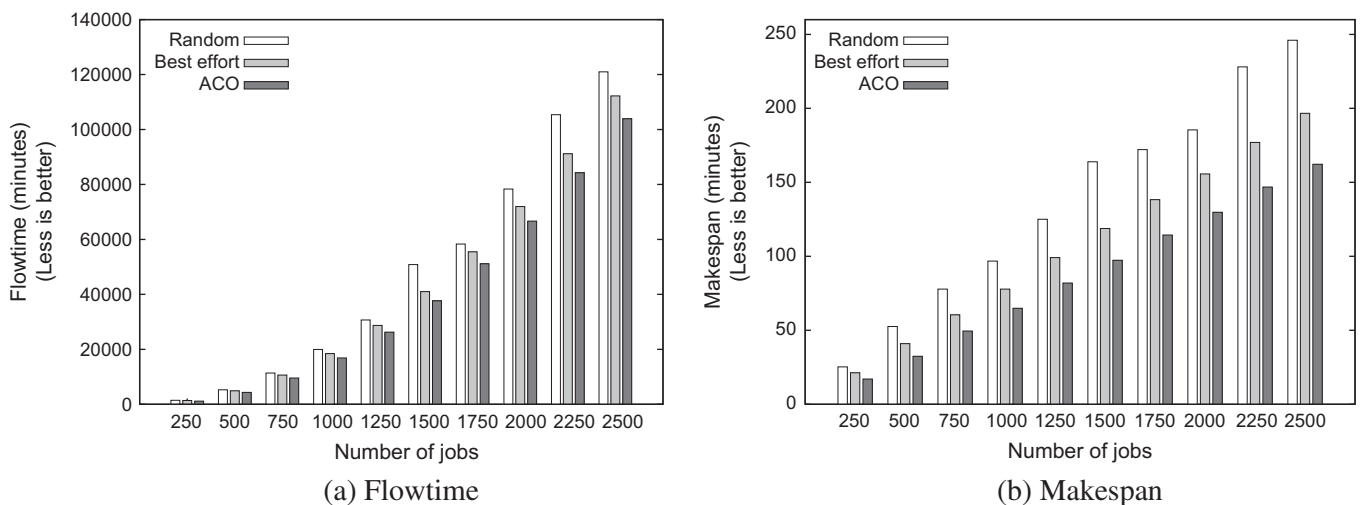
Fig. 6. Results as the number of jobs increases: Mesh of 1152 elements.
