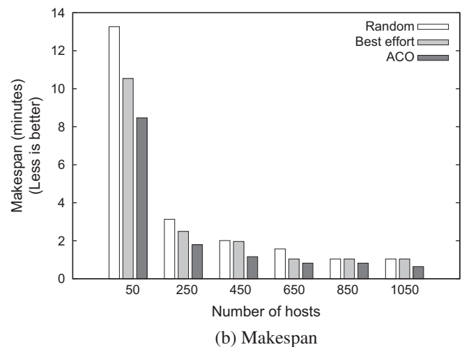
Fig. 7. Results as the number of hosts increases: Mesh of 288 elements.
