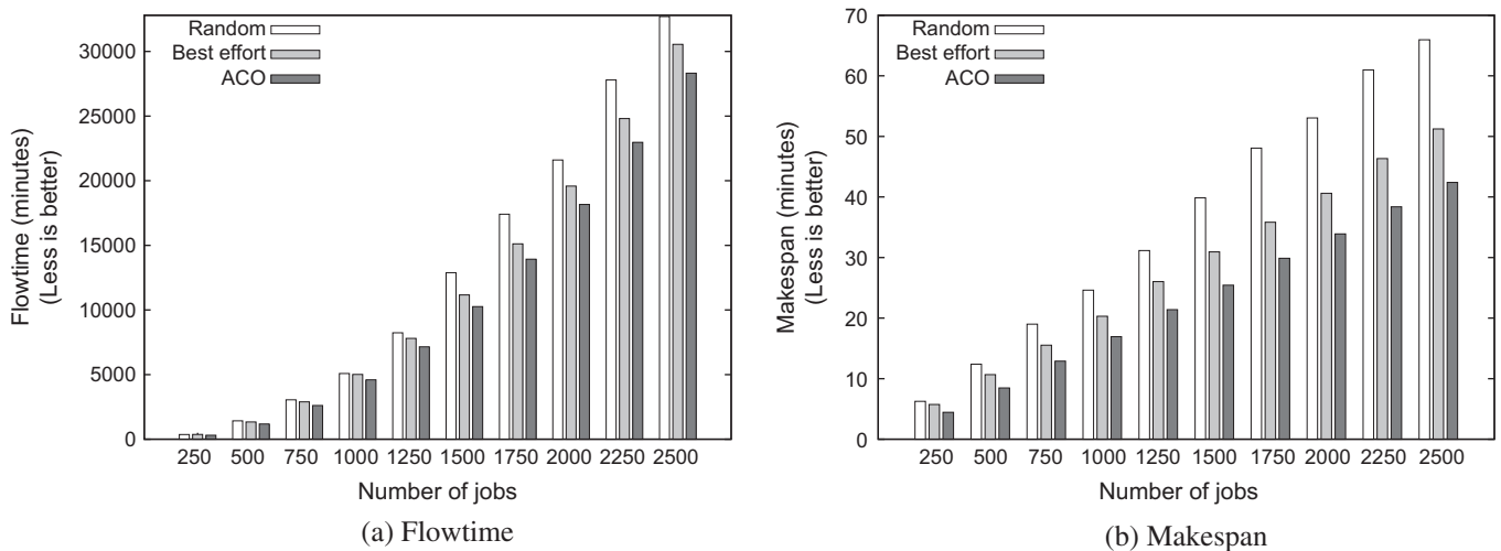
Fig. 5. Results as the number of jobs increases: Mesh of 288 elements.
