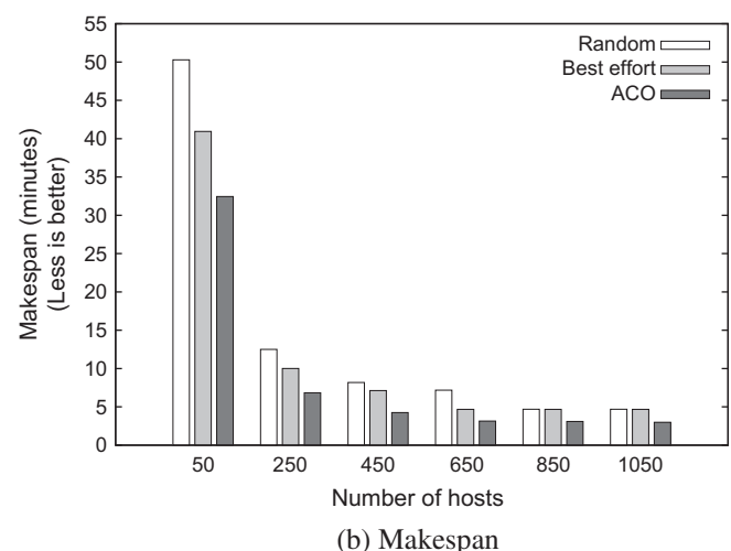
Fig. 8. Results as the number of hosts increases: Mesh of 1152 elements.
