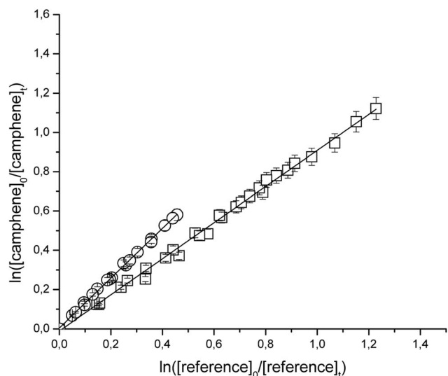
Fig. 2 Relative rate data for the reaction of Cl with camphene using isobutene ( \square ) and propene ( \circ ) as reference compounds at 298 K and atmospheric pressure of air.
