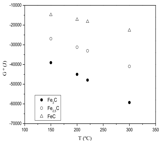
Fig. 6. Iron carbides stability in relation with temperature, predicted by thermodynamic simulation.
