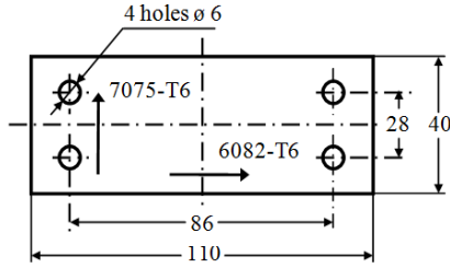
Fig. 2: Test specimen. The units are in mm, and the thickness is 4 mm
