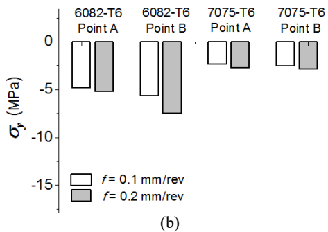
Fig. 4: Components; (a): \sigma_x and (b): \sigma_y of the residual stress (cutting speed: V = 1000 m/min, depth of cut: d = 1.5 mm)
