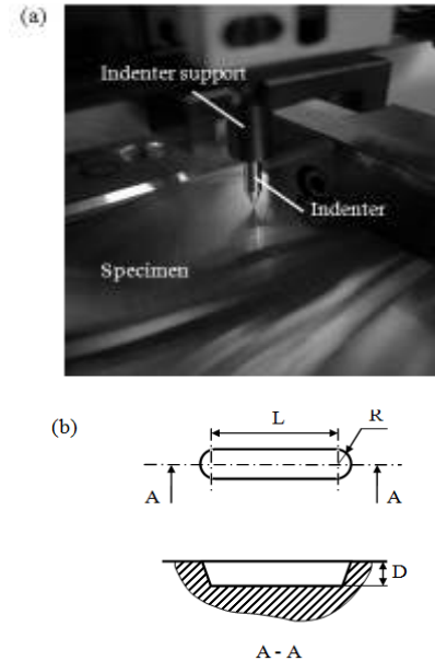
Fig. 1: (a): Picture of indenter-specimen interaction and (b): cross-section view of an elongated indent: (L) indent length; (R) end radius; (D) indent depth
