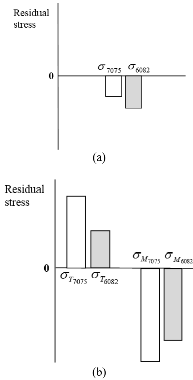
Fig. 6: (a): Global and (b): thermal and mechanical levels corresponding to normal components of residual stress
