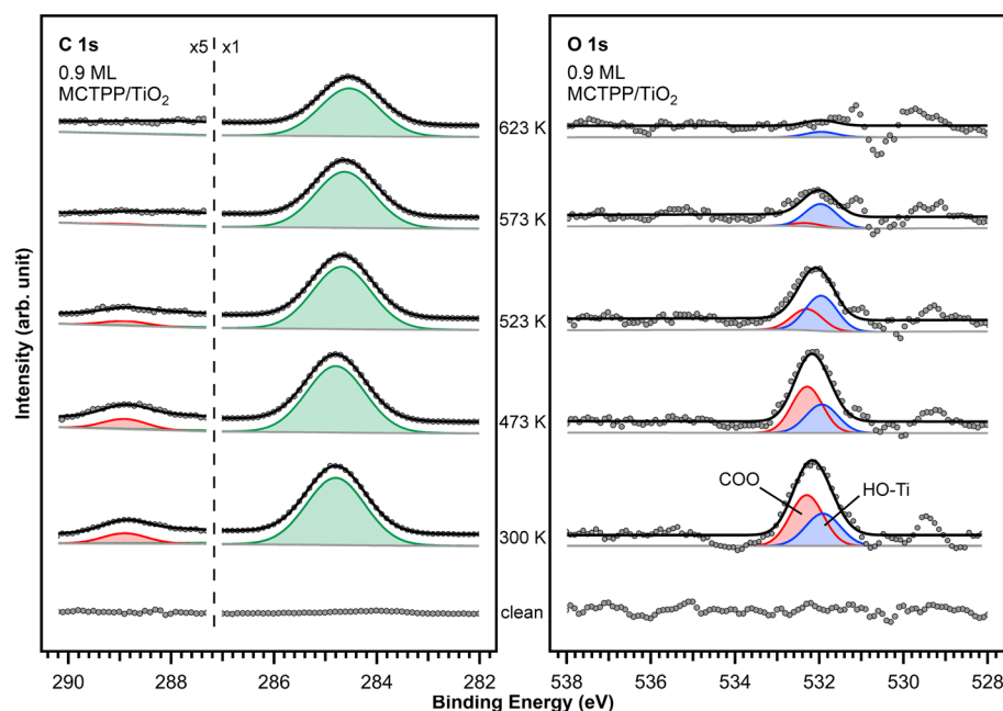
Figure 3. C 1s and O 1s spectra of 0.9 ML MCTPP on \text{TiO}_2(110) at room temperature and annealed to the indicated temperatures for 10 min. The carbon shakeup satellite and substrate oxygen peak have been removed for better clarity (see Figure 2). At elevated temperature, first the carboxylate groups and then the hydroxyl groups decompose.
