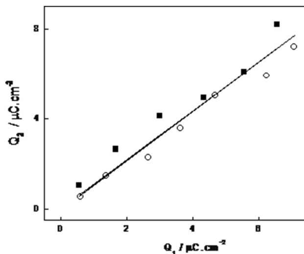
Figure 4. Comparison of charges involved in the \text{H}^+/\text{H}_2 couple on deposited Cd ( Q_2 ) and the charge involved in the cadmium UPD ( Q_1 ) for cathodic (■) and the anodic (○) processes. Charges were calculated from the data in Figure 3. The slope equals 1.09.
