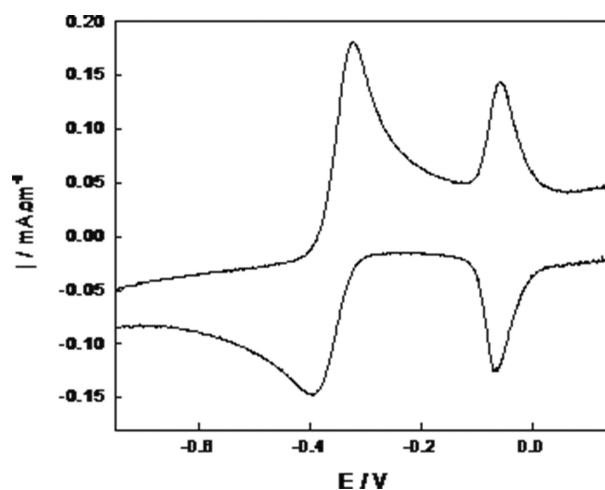
Figure 5. CV response of a dispersion of 15 nm gold nanoparticles (40 nM) at a HMDE in the presence of 0.11 mM Cd(II) (pH 2); Scan rate 1 \text{V s}^{-1} .
