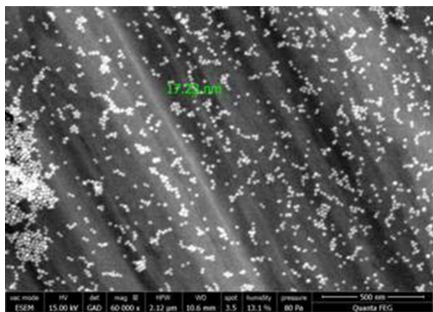
Figure 2. 15 kV Backscattered electron image in ESEM mode showing Au nanoparticles, here of ca. 17 nm in diameter, adsorbed on a mercury surface.
