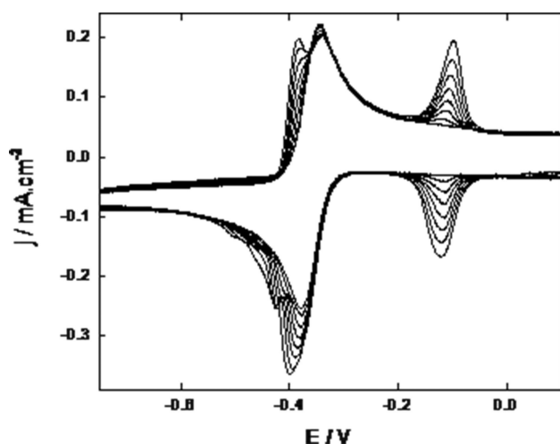
Figure 3. CVs recorded during nanoparticles adsorption on mercury in the presence of Cd(II). Conditions are indicated in Figure 1.
