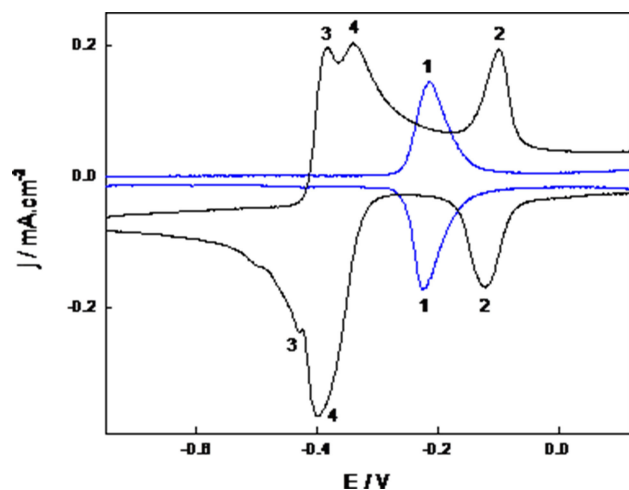
Figure 1. CV response of a dispersion of 15 nm gold nanoparticles (40 nM) at a HMDE in aqueous acetic acetate buffer (0.1 M, pH 4.5) in the absence of cadmium (blue line) and after Cd(II) addition (black line, 0.11 mM final concentration). Scan rate: 1 V s -1 . Potentials are quoted against NHE.
