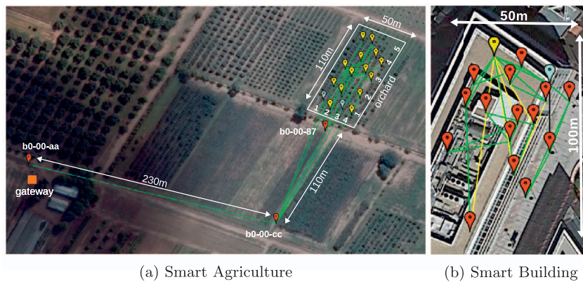
Fig. 3. Aerial view of the topology of both deployments. The deployment is done in both cases in roughly a 50 m \times 100 m area.
