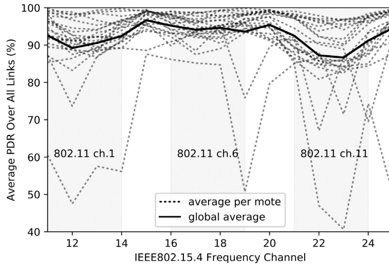
Fig. 6. In the Smart Building deployment, external interference from nearby WiFi devices causes some retries (the PDR is lower) without impacting end-to-end reliability which stays at 100% (see Section 5.3).
