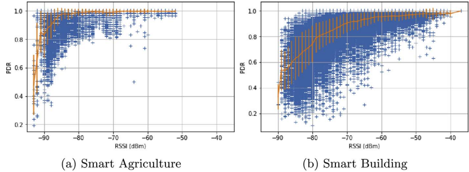
Fig. 5. The PDR/RSSI “waterfall” plot. The Smart Building plot is shifted right compared to the Smart Agriculture plot, indicating an environment where external interference is present.
