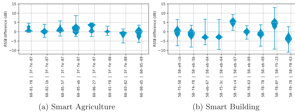
Fig. 7. The difference in RSSI between the two directions of the wireless links with the highest number of exchanged messages. The violin plots show the distribution of the value and the standard deviation.
