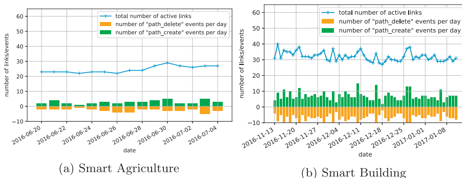
Fig. 8. Network stability: the number of path_create and path_delete events generated per day over a 16 day (Smart Agriculture) and two month (Smart Building) period. The top line shows the total number of active links.
