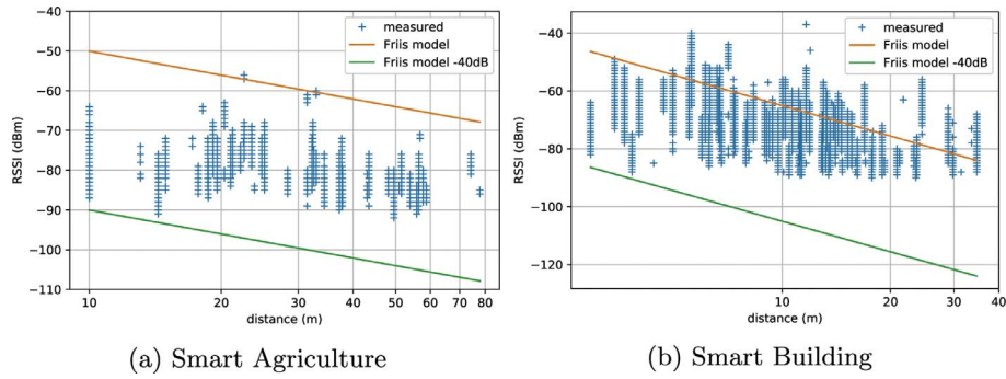
Fig. 4. We observe that the RSSI measurements are roughly located between the Friis model and the Friis model shifted by -40 dB.
