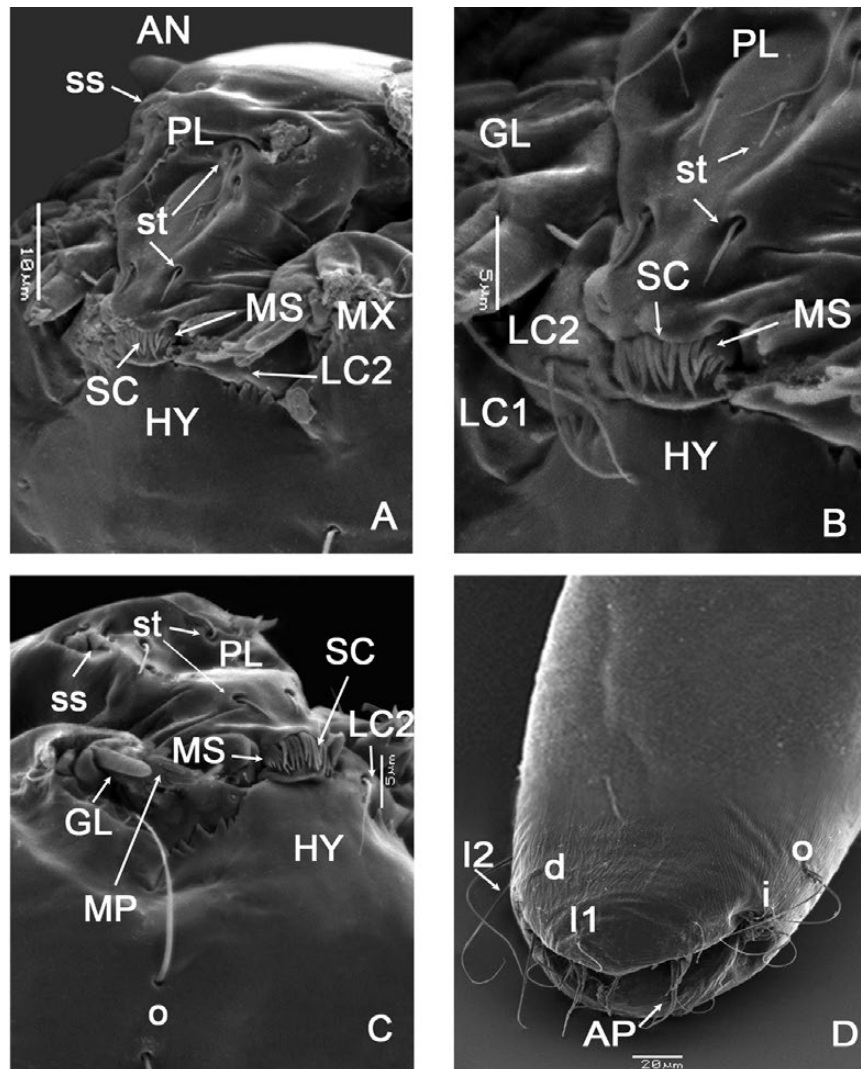
Fig. 2. Scanning electron micrographs of larva Culicoides trilineatus Fox (Diptera: Ceratopogonidae) collected in Argentina: palatum, messors, and scope (A); detail palatum (B); detail maxilla (C); caudal segment, dorsal view (D). AN, antennae; AP, anal papillae; GL, galeolacinia; HY, hypostoma; LC2, lacinial sclerite 2; LCT, lateral curtains; MD, mandible; MX, maxilla; MP, maxillary palpus; MS, messors; PL, palatum; SC, scopae; ss, sensilla styloconica; st, sensilla trichoidea. Caudal segment chaetotaxy: 'd', dorsal setae; 'i', inner seta; 'l 1 ', first lateral seta; 'l 2 ', second lateral seta; 'o', outer seta; 'p', posterior perifrontal seta; 'q', postfrontal setae; 'v', ventral setae.
