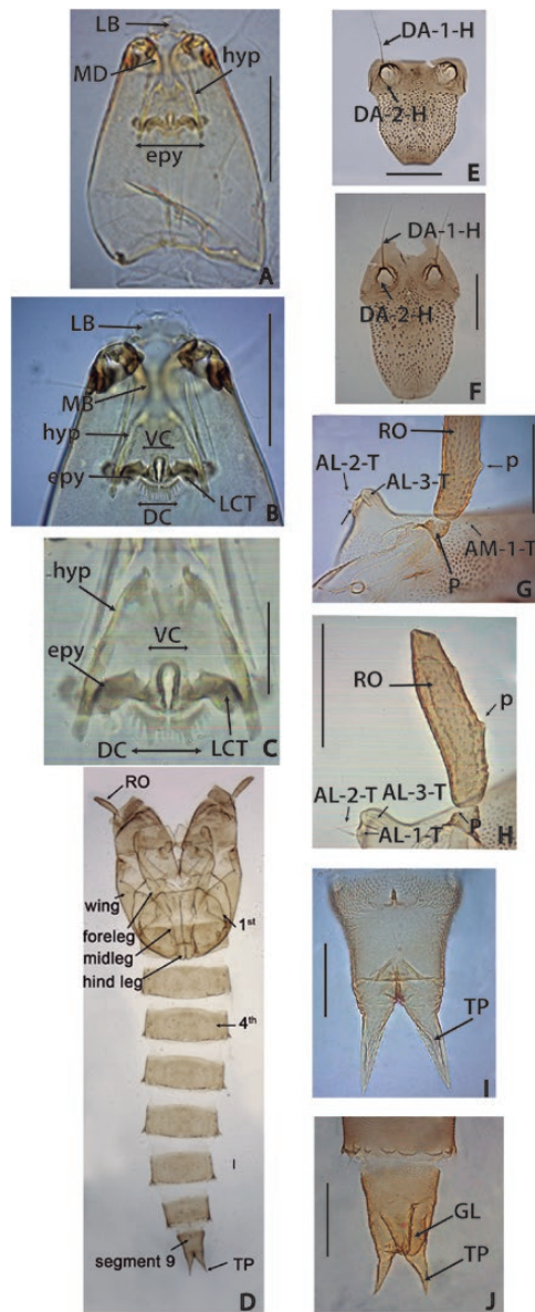
Fig. 3. Larva and pupa of Culicoides trilineatus Fox (Diptera: Ceratopogonidae) collected in Argentina: Larva (A-C); female pupa (D-E, I); male pupa (F-H, J); head capsule (A); head capsule, anteroventral view (B); detail epipharynx (C); entire pupa (D); dorsal apotome (E-F); anteromedial and anterolateral sensilla (G); respiratory organ (H); segment 9 (I-J). AL-1-T, AL-2-T, AL-3-T, anterolateral sensilla; AM-1-T, AM-2-T, AM-3-T, anteromedial sensilla; DA-1-H, D-2-H, dorsal apotome sensilla; DC, dorsal comb; epi, epipharynx; GL, genital lobe; hyp, hypopharynx; LTC lateral curtains; MD, mandible; LB, labrum; P, pedicel; p, pore; RO, respiratory organ; TP, terminal process; VC, ventral comb.
