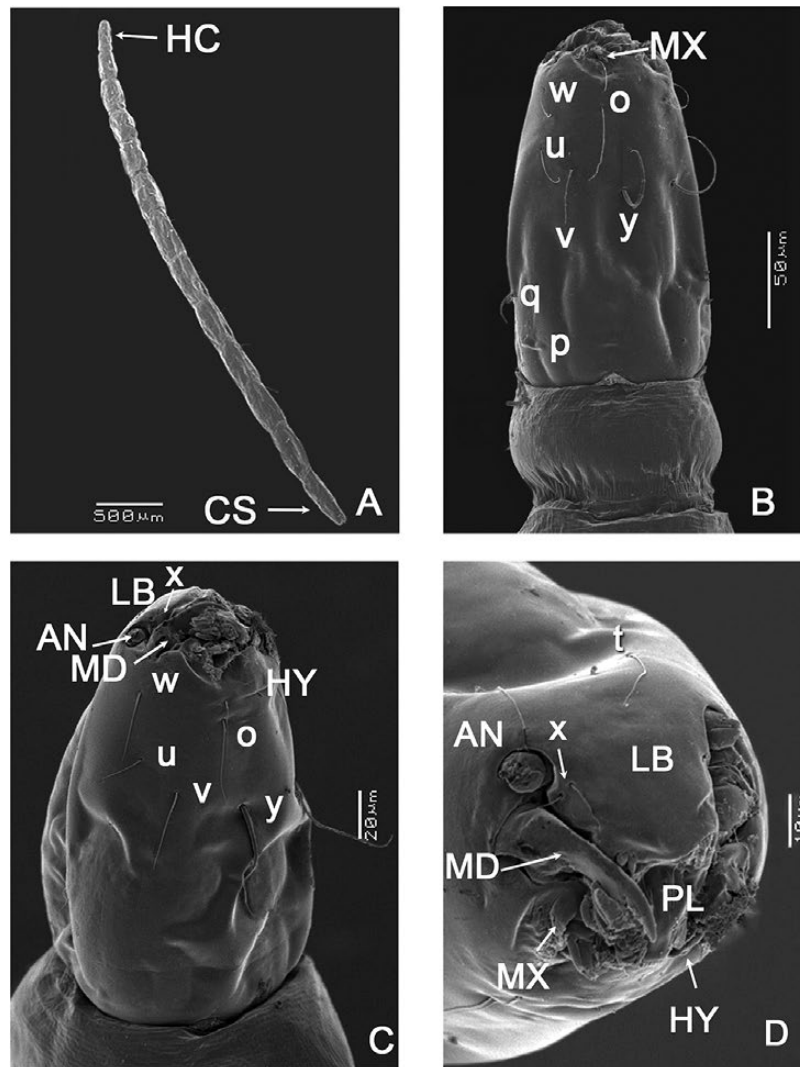
Fig. 1. Scanning electron micrographs of larva Culicoides trilineatus Fox (Diptera: Ceratopogonidae) collected in Argentina: entire larva (A); head capsule, lateroventral view (B); head capsule, ventral view (C); head capsule, laterofrontal view (D). AN, antennae; CS, caudal segment; GL, galeolacinia; HC, head capsule; HY, hypostoma; LB, labrum; MD, mandible; MX, maxilla; PL, palatum; ss, sensilla styloconica; st, sensilla trichoidea. Head capsule chaetotaxy are indicated by single letters: o, parahypostomal setae; t, prefrontal setae; u, mesolateral setae; v, posterolateral setae; w, anterolateral setae; x, parantennal setae; y, ventral setae.
