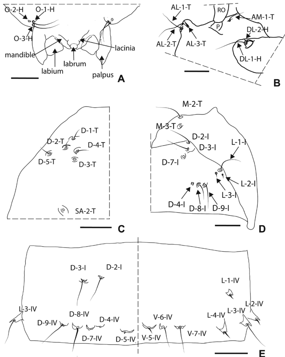
Fig. 4. Draw of pupa Culicoides trilineatus Fox (Diptera: Ceratopogonidae) collected in Argentina: Female pupa (A, C–E); male pupa (B): Mouthparts and ocular sensilla (A); Cephalothoracic sensilla (B); dorsal sensilla (C); metathorax and tergite 1 (D); segment 4 (E). Scale bars: 0.05 mm. AL-1-T, AL-2-T, AL-3-T, anterolateral sensilla; AM-1-T, anteromedial sensilla; D-1-T, D-2-T, D-3-T, D-4-T, D-5-T, dorsal sensilla; DL-1-H, DL-2-H, dorsolateral cephalic sclerite sensilla; M-2-T, M-3-T, metathoracic sensilla; O-1-H, O-2-H, O-3-H, ocular sensilla; P, pedicel; RO, respiratory organ; D-1-IV, D-2-IV, D-3-IV, D-4-IV, D-5-IV, D-7-IV, D-8-IV, D-9-IV, L-1-IV, L-2-IV, L-3-IV, L-4-IV, V-1-IV, V-5-IV, V-6-IV, V-7-IV, segment 4 sensilla; D-1-I, D-2-I, D-4-I, D-7-I, D-8-I, D-9-I, L-1-I, L-2-I, L-3-I, tergite 1 sensilla.
