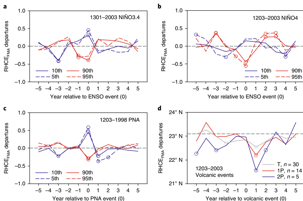
Fig. 3 | RHCE FMA response to ENSO and PNA extremes and to major volcanic events. a–c, SEAs showing RHCE FMA anomalies during extreme negative (positive) El Niño Southern Oscillation (ENSO) and Pacific-North American years, defined as the 5th and 10th (95th and 90th) percentiles of two ENSO reconstructions, NIÑO3.4 SST 24 ( a ) and NIÑO4 SST 25 ( b ), and one PNA reconstruction 26 ( c ). d, SEA showing the RHCE FMA response in degrees of latitude to tropical volcanic events (T) and events the same size as Pinatubo (1P) or twice as large (2P), based on a revised volcanic forcing reconstruction 29 . Significant ( P < 0.05 ) departures are indicated by circles. The list of the events is in Supplementary Tables 4 and 6.
