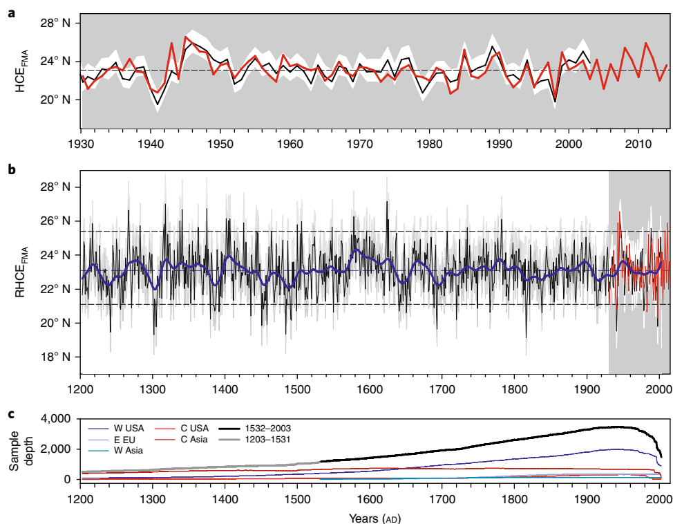
Fig. 2 | Reconstruction of the early spring northern boundary of the tropical belt. a, b, Annually resolved instrumental (red line, HCE FMA ) and reconstructed (black line, RHCE FMA ) February–April Hadley circulation extent in degrees of latitude for the AD 1930–2014 instrumental period ( a ) and the AD 1203–2003 period ( b ). In b , the blue line represents the 30-year low-pass-filtered RHCE FMA , and dashed horizontal lines indicate the average, 5th and 95th percentile positions of RHCE FMA . Shading around the reconstruction represents the combined chronology and calibration error estimation. c, Sample depth over time for each of the five master chronologies and for the periods AD 1532–2003 and AD 1203–1531.
