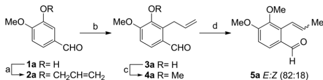
Scheme 2. Reagents and conditions: a) \text{BrCH}_2\text{CH}=\text{CH}_2 , \text{K}_2\text{CO}_3 , EtOH, reflux, 3 h (93 %); b) 1,2- \text{Cl}_2\text{C}_6\text{H}_4 , 180 °C, 20 h (90 %); c) MeI, \text{K}_2\text{CO}_3 , EtOH, reflux, 6 h (95 %); d) \text{RuCl}(\text{CO})(\text{PPh}_3)_3 , PhMe, 80 °C, 24 h (90 %).
