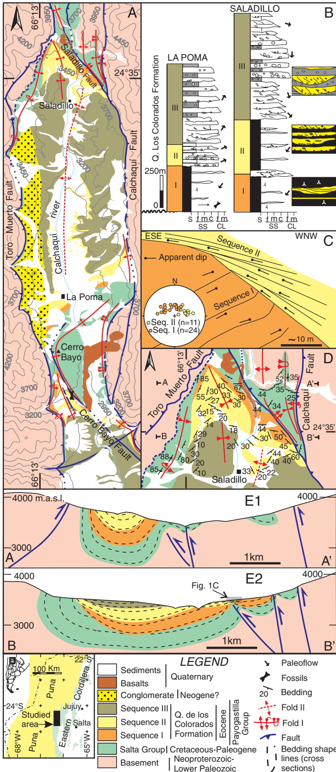
Figure 1. A: Geologic map of North Calchaquí Valley. B: Columns of Quebrada de los Colorados Formation in Saladillo and La Poma; schematic facies stacking is represented. C: Syntectonic angular unconformity between sequences I and II. Stereonet shows poles to bedding in both sequences. D: Geology of Saladillo area. E: Profiles of Saladillo syncline (profile locations in D).
