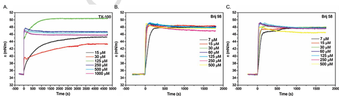
Fig. 4. Binding kinetics of detergents to Langmuir films of lipids extracted from erythrocyte ghosts : TX-100 (A), Brij 98 (B) and Brij 58 (C); temperature = 22 °C.
