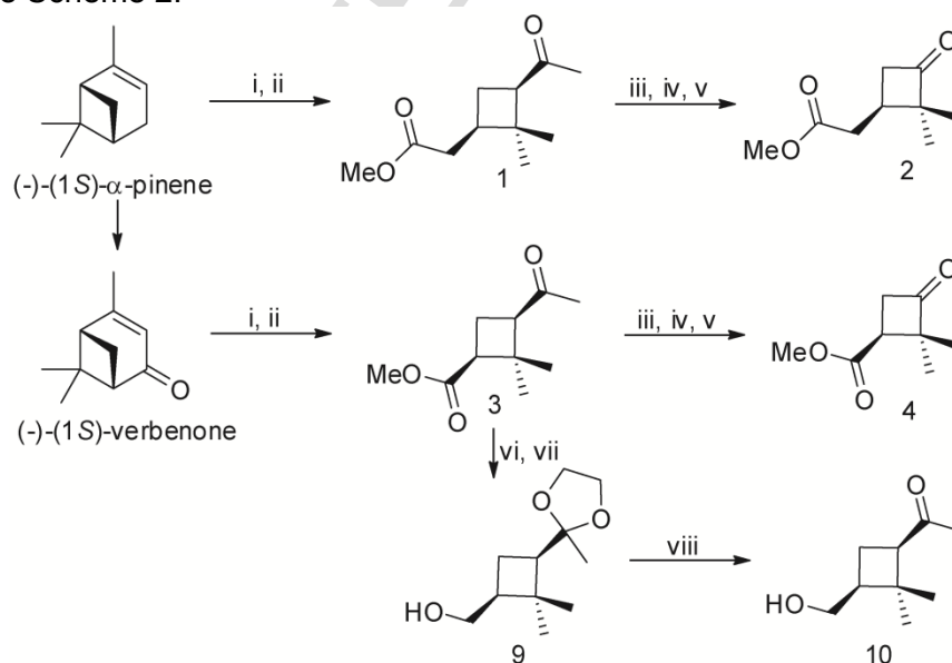
Scheme 2. Synthesis of ketones 1-4 and 10 . Reagents and conditions: i) \text{NaIO}_4 , \text{RuCl}_3 , \text{H}_2\text{O}/\text{CH}_3\text{CN}/\text{CCl}_4 , rt; ii) \text{CH}_2\text{N}_2 , \text{Et}_2\text{O} , 50^\circ\text{C} ; iii) m -CPBA, \text{CH}_2\text{Cl}_2 , rt; iv) \text{K}_2\text{CO}_3 , \text{H}_2\text{O}/\text{MeOH}/\text{THF} , rt; v) DMP, \text{CH}_2\text{Cl}_2 , rt; vi) (\text{CH}_2\text{OH})_2 , PPTS, PhH, reflux; vii) \text{LiBH}_4 , THF, rt; viii) PPTS, (\text{CH}_3)_2\text{CO} , 56^\circ\text{C} .
