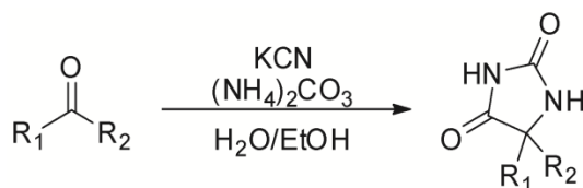
Scheme 1. General procedure to obtain hydantoins from carbonyl compounds
