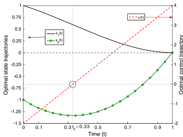
Figure 1. Optimal states and control trajectories for the ‘cheapest stop of a train’ problem with unbounded control values and hard endpoint restriction x(T) = (0, 0)' .
