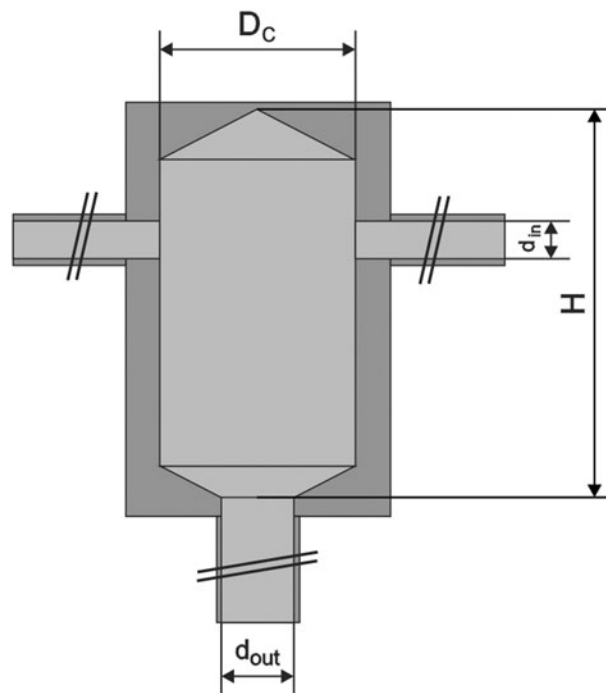
Figure 2. Scheme of the confined impinging jet mixer used. D_c=4.8 mm, d_{in}=1 mm, d_{out}=2 mm; H is approximately equal to 2D_c .
