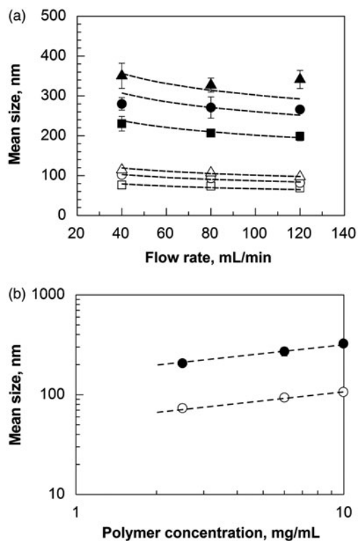
Figure 3. Mean size of PCL (filled symbols) and PLGA (empty symbols) nanoparticles obtained (a) under different flow rates for (■,□) 2.5, (●,○) 6 and (▲,△) 10 mg/mL of polymer, and (b) under different polymer concentrations at flow rate 80 mL/min. The trend lines were calculated using Equation (3), with \alpha = 0.29 and \beta = -0.18 ; error bars in Figure 3 (b) are smaller than symbols.
