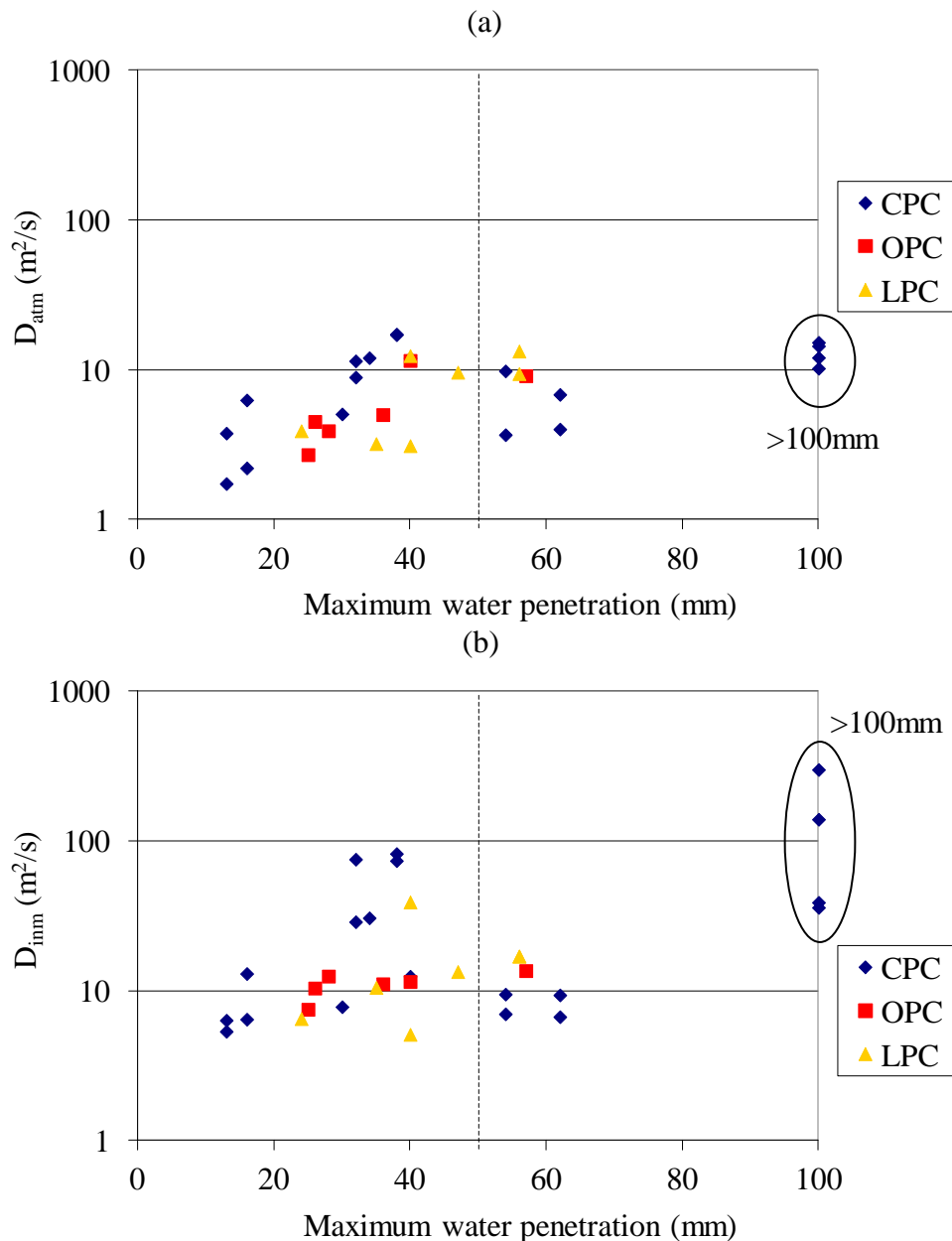
Figure 6. (a) D_{atm} and (b) D_{inm} vs maximum penetration of water under pressure.
