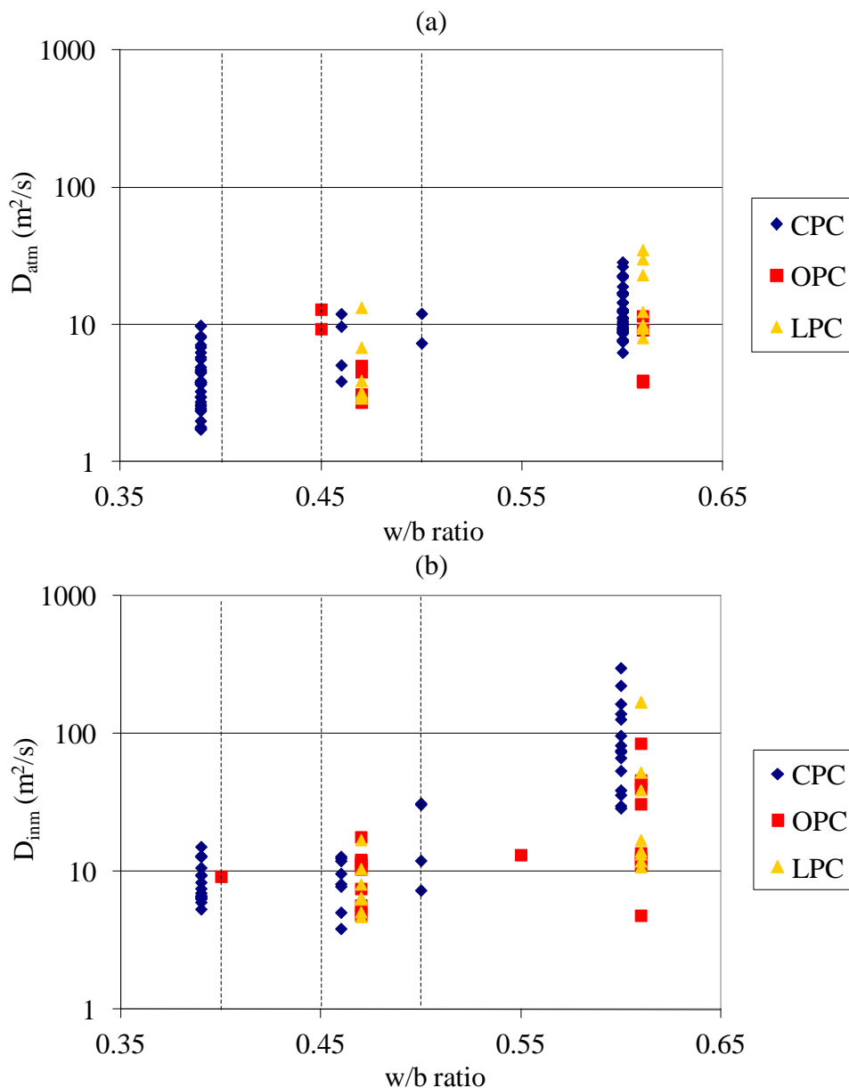
Figure 2. (a) D_{atm} and (b) D_{inm} , versus w/b.
