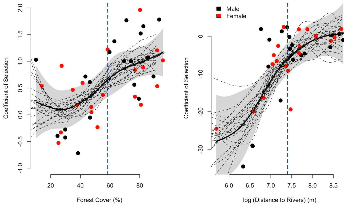
Fig. 3. The left panel is the estimate of the smooth function (black line) and 30 smooth curves drawn from the posterior (dotted lines) of a generalized additive model considering the coefficient of selection in relation to forest cover (%). The gray area indicates the 95% CI. The blue dashed line is the shifting point (58.4%). Notice the uncertainty of the response at low forest coverage and the tendency for jaguars in heavily-forested landscapes to more strongly avoid non-forest. The right panel is the estimate of the smooth function (black line) and 30 smooth curves drawn from the posterior (dotted lines) of a generalized additive model considering the coefficient of selection in relation to log distance to water (m). The blue dashed line is the shifting point (1685 m). The gray area indicates the 95% CI. Notice that jaguars further from watercourses move independently of water location. (For interpretation of the references to colour in this figure legend, the reader is referred to the web version of this article.)
