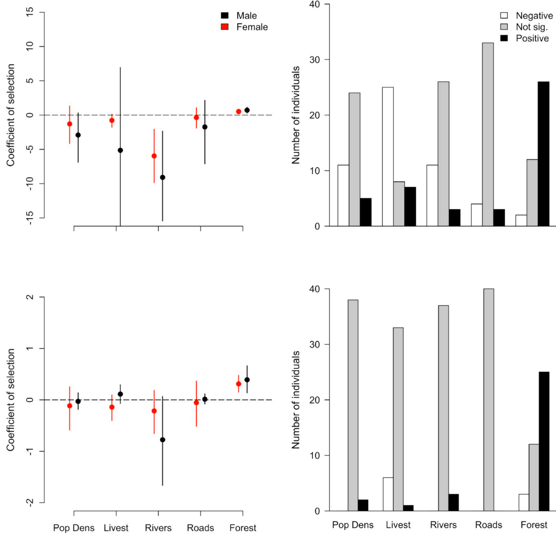
Fig. 2. Estimated overall selection coefficients by gender for each resource variable for the home range scale (top left) and foraging scale analysis (bottom left) (Points = Posterior Mean, lines = 95% HPDI interval). Number of jaguar showing positive, negative, or non-significant relationships for each habitat variable at the home range (top right) and foraging scale (bottom right) (based on 95% HPDI overlapping zero or not). Pop Dens = Human population density per km 2 , Rivers = distance to rivers (m), Livest = livestock density per km 2 , Roads = distance to roads (m) and Forest = forest cover (%).
