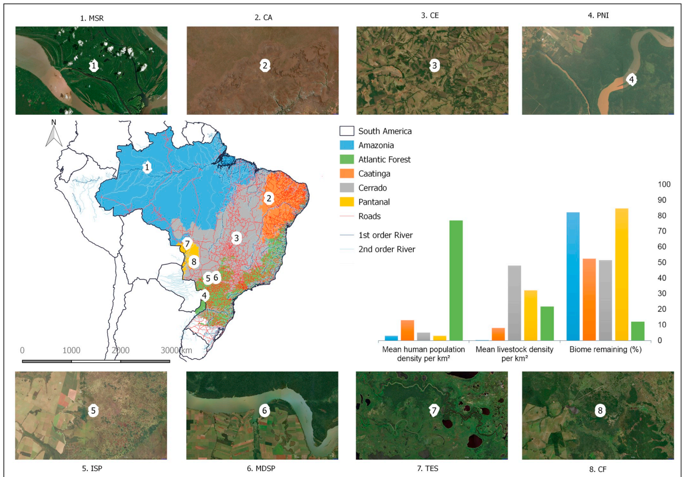
Fig. 1. Map of study area locations and associated aerial images depicting landscape characteristics of each study site. Histograms indicate mean human population density per km 2 , mean livestock density per km 2 and % of biome remaining. Study sites were: 1) Mamirauá Sustainable Reserve (MSR, Amazon), 2) Serra da Capivara National Park (CA, Caatinga), 3) private lands at the Cerrado (CE), 4) Iguazú and Iguacu National Parks (PNI, Atlantic Forest), 5) Invinhema State Park (ISP, Atlantic Forest), 6) Morro do Diabo State Park (MDSP, Atlantic Forest); 7) Taiama Ecological Station (TES, Pantanal); 8) Caiman Farm (CF, Pantanal).
