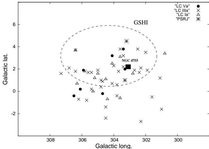
Fig. 12. Members of CenOB1 in galactic coordinates. The luminous classes of the stars are indicated with different symbols (upper-right corner). The asterisks mark the location of the pulsars. The dashed ellipse represents the HI shell GS305+04-26 (Corti et al. 2012). The NGC 4755 cluster is indicated with a black box.
