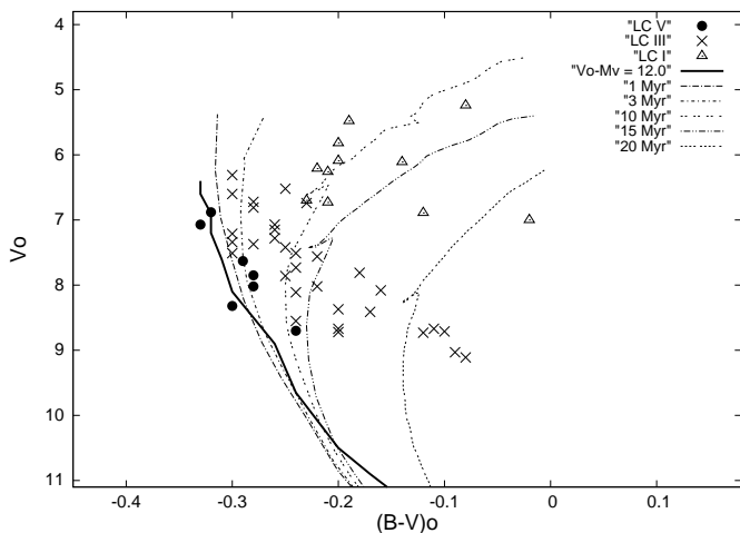
Fig. 13. CMD of member stars of Cen OB1. The symbols are the same as in Fig. 12. The black curve is the Schmidt-Kaler (Th. 1982) HR diagram for early stars; the other curves are Marigo et al. (2008) isochones for z = 0.02 . All the reference curves are corrected by an apparent distance modulus of 12.0
