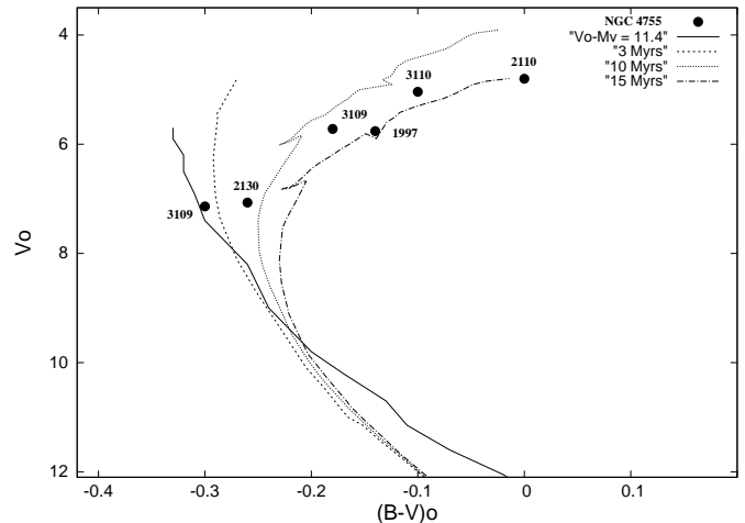
Fig. 14. CMD of member stars of NGC 4755. The symbols are the same as in Fig. 12. The black curve is the Schmidt-Kaler (Th. 1982) HR diagram for early stars; the other curves are Marigo et al. (2008) isochones for z = 0.02 . All the reference curves are corrected by an apparent distance modulus of 11.4
