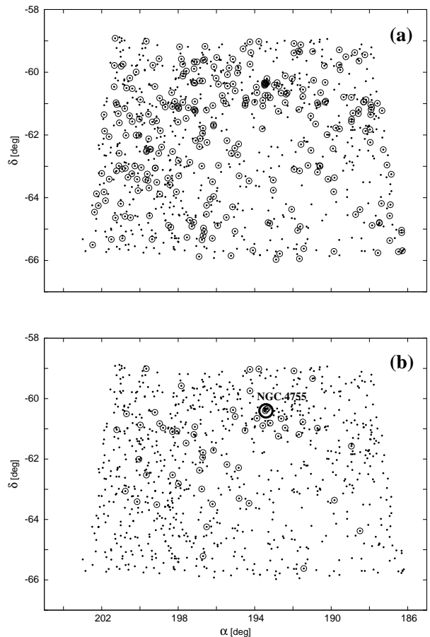
Fig. 3. Spatial distribution of the stellar association Cen OB1. (a) Open circles around the dots represent the 299 astrometric association members; the points represent the rest of the stars of the region in the first analysis. (b) Open circles represent the 52 astrometric and spectrophotometric association members obtained using the model proposed by Orellana et al. (2010). The NGC 4755 cluster is indicated by the large circle.
