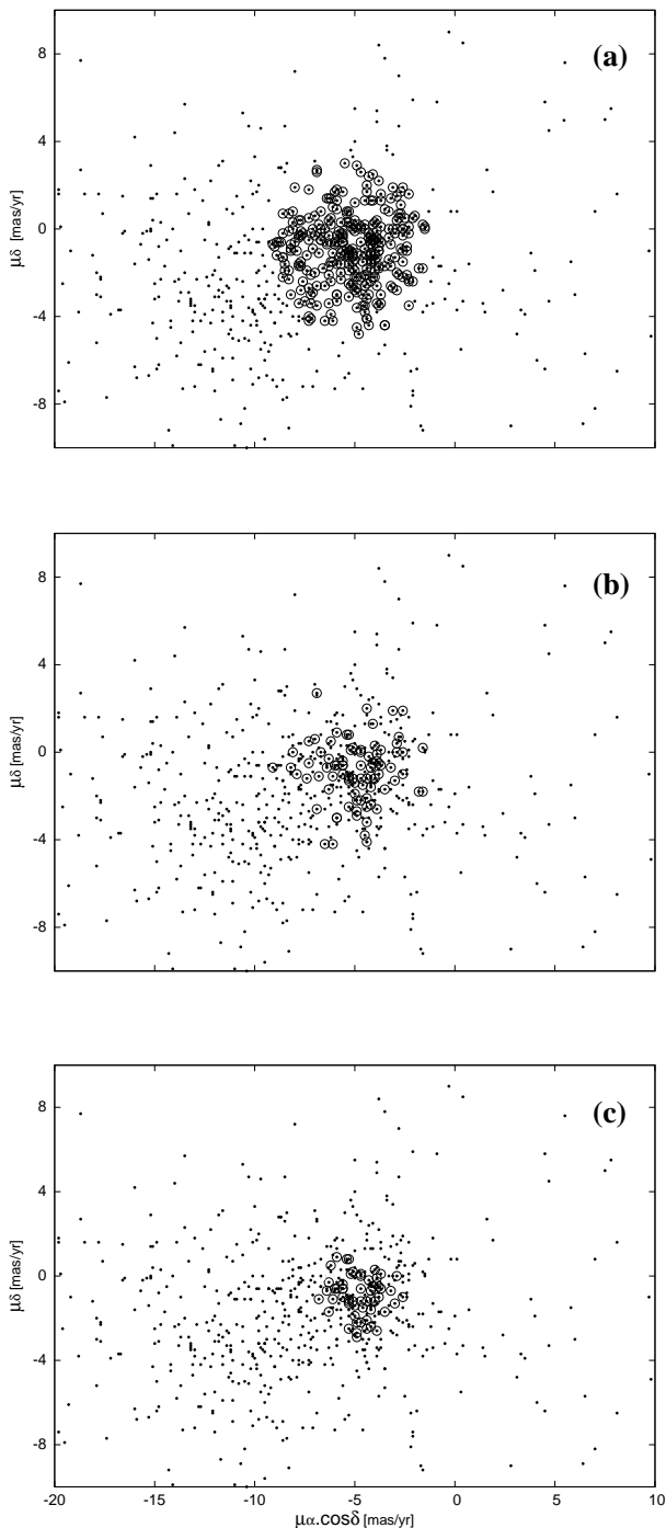
Fig. 4. VPD of the stellar association Cen OB1. (a) Open circles around the dots represent the 299 astrometric association members; points represent the rest of the stars of the region in the first analysis. (b) Open circles represent the 86 astrometric and spectrophotometric members. (c) Open circles represent the 52 astrometric and spectrophotometric association members obtained using the model proposed by Orellana et al. (2010).
