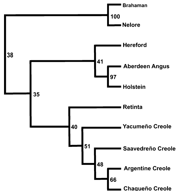
Figure 1. UPGMA tree of genetic relationships among 10 cattle breeds using D_A genetics distances. The numbers on nodes are percentage bootstrap values in 1000 replications.
