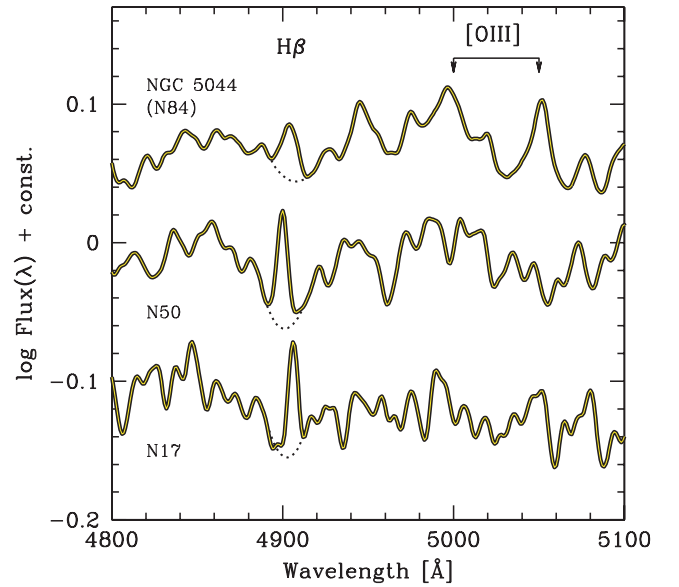
Figure 17. An H\beta gas emission component, superposed to the stellar absorption is clearly evident in the spectra of the three ellipticals NGC 5044 (alias N84), N50 and N17. Note, for the latter cases, that no sizeable [O III] emission is detected at the expected (rest-frame) wavelength of 4959 and 5007 Å, as labelled. The envisaged (conservative) correction to H\beta , as explained in the text, is indicated here by the dashed curves.
