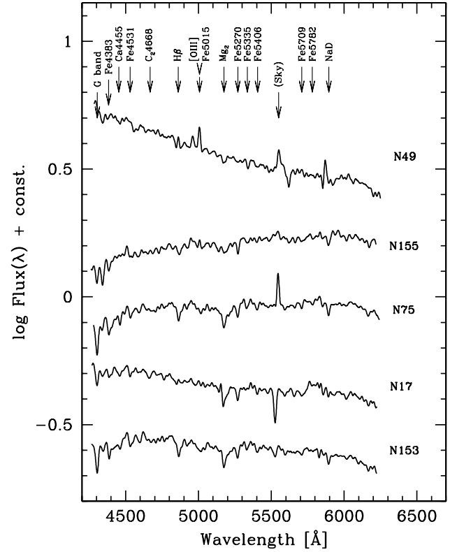
Figure 13. Same as Fig. 11, but for a second set of member galaxies observed at ESO. Note the outstanding H\beta and [O\text{III}] 5007 \text{ \AA} emission in Im galaxy N49. For easier reading, spectra have been degraded here to a resolution of 12 \text{ \AA} FWHM and corrected for redshift. Marked at the top are also all the main spectral features included in the Lick narrow-band index system (see Table 8).
