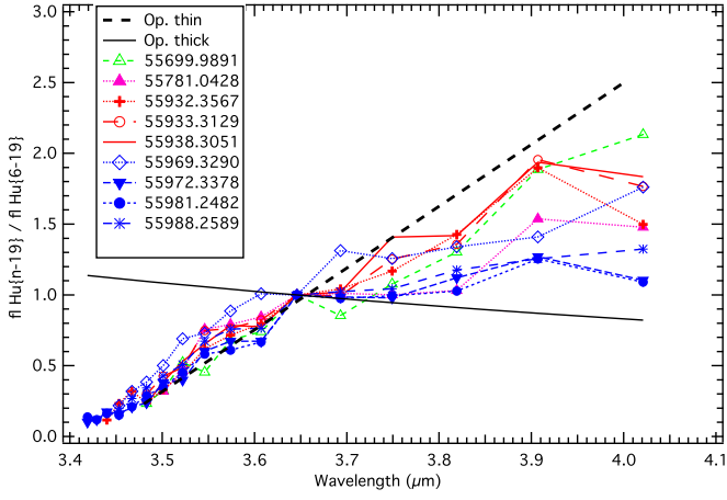
Figure 6. Line flux ratios of Humphreys' lines relative to \text{Hu}_{19} . Different symbols indicate different epochs. The optically thin case is represented with a dashed straight line, and the optically thick case with a solid line.
