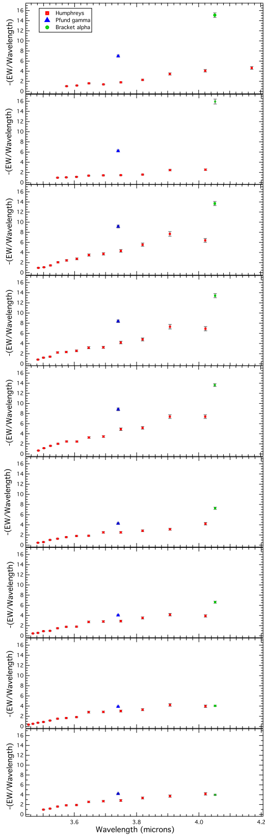
Figure 4. EW/\lambda vs. wavelength for Br\alpha , Pf\gamma , and Humphrey lines. The first observation corresponds to the lower frame and time direction goes upwards.
