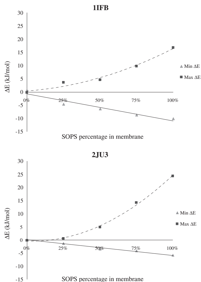
Fig. 3. Electrostatic free energy of IFABP and LFABP vs POPC:SOPS ratio. Values corresponding to most favorable configurations ( \blacktriangle ) have soft and lineal decreasing; while less favorable relative positions ( \blacksquare ) increase exponentially nominal values of free interaction energy.
