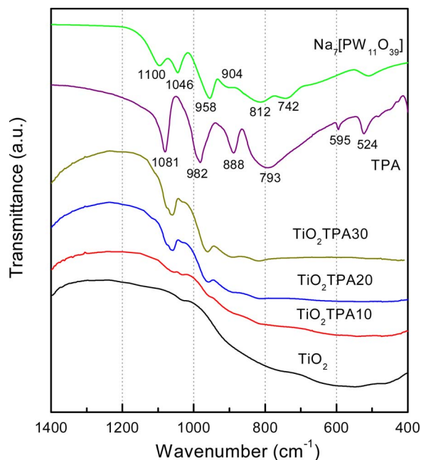
Fig. 6. Infrared spectra of the composite and reference materials (bulk TPA and Na 7 [PW 11 O 39 ]).
