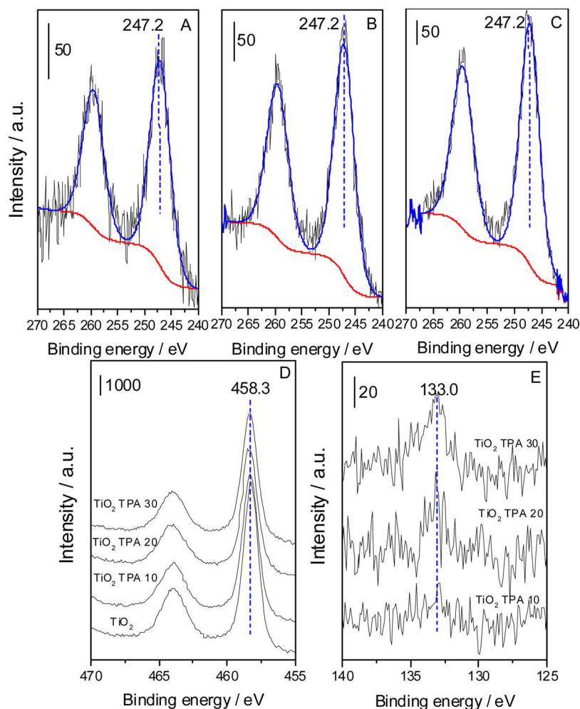
Fig. 5. W 4d XPS spectra of the TiO 2 TPA10 (A), TiO 2 TPA20 (B) and TiO 2 TPA30 (C) sample, respectively. (D) Ti 2p XPS spectra of the TiO 2 TPA(X) samples and Ti references. (E) P 2p XPS spectra of the TiO 2 TPA(X) samples.
