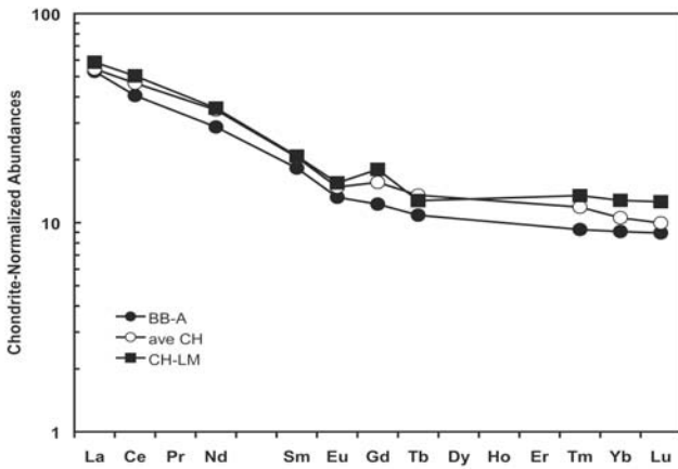
Fig. 7. Distribution of rare earth elements (REE) for average CH glasses (open circles), BB glass (filled circles), and host CH sediments (filled squares). The impact glasses exhibit a smaller Eu anomaly consistent with a source more mafic than the host sediments.
