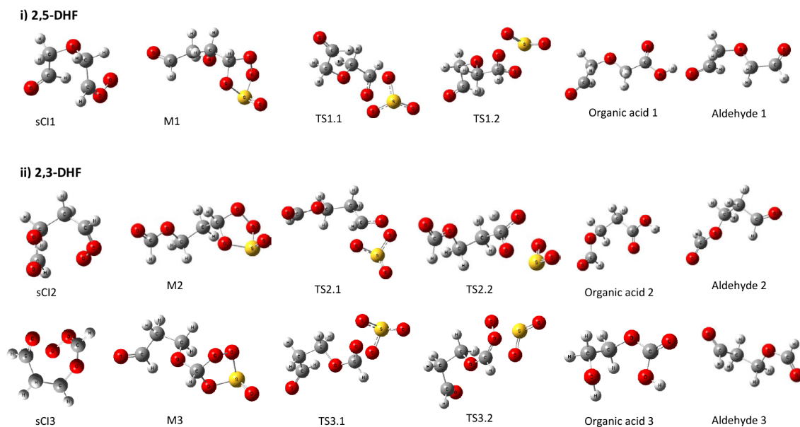
Figure 5. (a) General schematic potential energy surface for the reactions sCI + SO_2 \rightarrow products. (b) Geometries of stationary points involved in the sCI + SO_2 reaction at the BMK/6-311++G(3df,3pd) level of theory.
