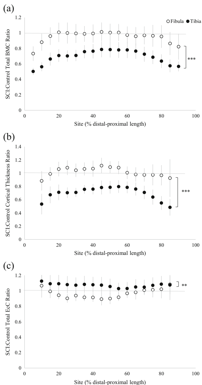
Fig. 3 Comparison of tibia and fibula a total BMC, b cortical thickness and c endocortical circumference group differences, as ratio of paired values \pm 95\% CI. Asterisks indicate the main effect of bone (tibia/fibula); ** P < 0.01 , *** P < 0.001
