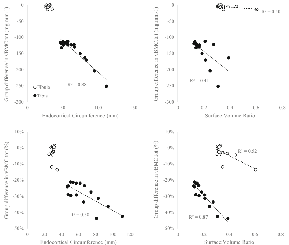
Fig. 4 Associations between absolute and relative (%) paired differences in total BMC (vBMC.tot) and endocortical circumference and surface/volume ratio at different sites throughout tibia and fibula. Association significant at P < 0.001
