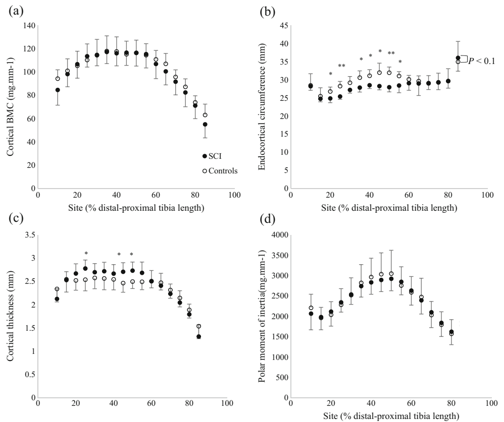
Fig. 2 Cortical geometry in SCI and controls, as mean \pm 95 % CI. Asterisks indicate location of significant site-specific group differences with respect to 80 % site as identified by site \times group interactions detailed in Table 1; * P < 0.05 , ** P < 0.01 , *** P < 0.001
