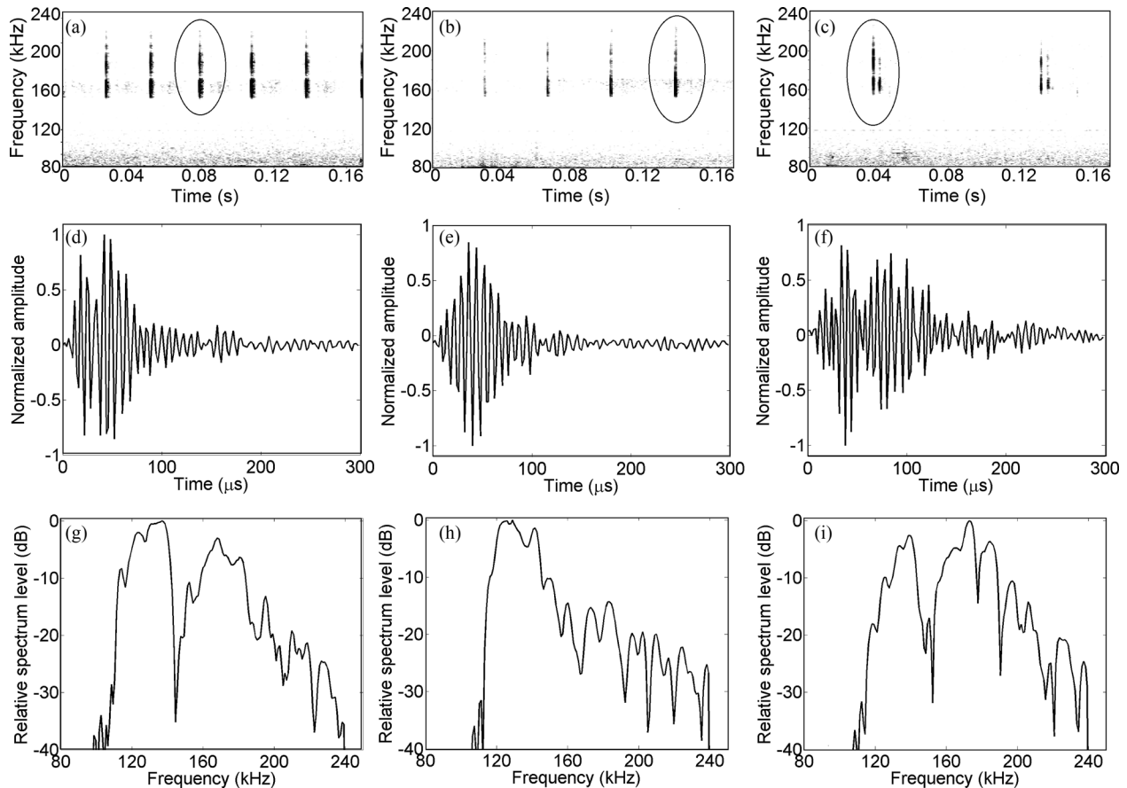
FIG. 4. Spectrogram of an echolocation click train (1024-point FFT, 0.002 s FFT length, 0% overlap, hamming window) showing a representative click (black circle), its time series and normalized spectrum (512-point FFT, 500 kHz sampling frequency, rectangular window) for each cluster. (a) and (d) cluster 1, (b) and (e) cluster 2, and (c) and (f) cluster 3.
