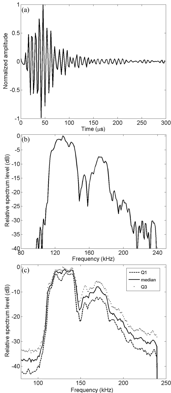
FIG. 5. (a) Normalized time series of a representative buzz click. (b) Normalized spectrum of a representative buzz click. (c) Normalized median spectrum with its lower ( Q1 ) and upper quartile ( Q3 ) of all buzz clicks analyzed (512-point FFT, 500 kHz sampling frequency, rectangular window).
