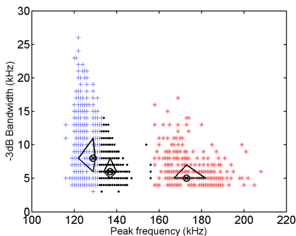
FIG. 3. (Color online) Peak frequency (kHz) of regular clicks within each cluster against the 3 dB bandwidth (kHz). Clicks within cluster 1 are represented by spots, cluster 2 by pluses, and cluster 3 by asterisks. The medians of each cluster are represented by a cross within a circle and the area inside the lines include clicks between the lower quartiles ( Q1 ) and upper quartiles ( Q3 ) of the distributions of the two parameters for each cluster.
