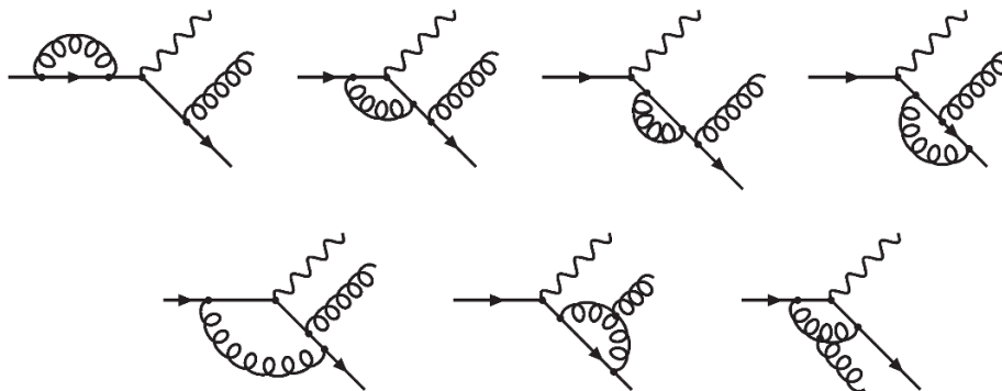
Figure 3. Representative Feynman diagrams contributing to the q \rightarrow qg\gamma splitting amplitude. The first 5 diagrams are associated with the Abelian contribution already presented in q \rightarrow q\gamma\gamma . The last 2 diagrams lead to non-Abelian (NA) contributions.
