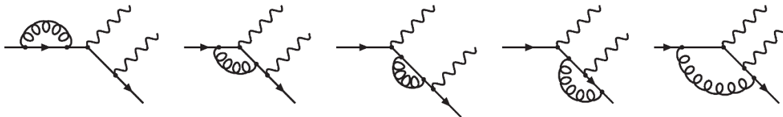
Figure 2. Representative Feynman diagrams contributing to the q \rightarrow q\gamma\gamma splitting amplitude. This splitting amplitude is symmetric under the exchange of the two final state photons.
