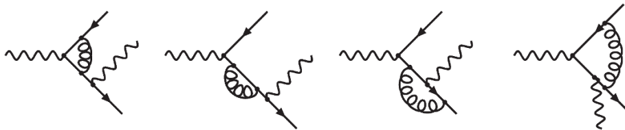
Figure 5. Representative diagrams contributing to the \gamma \rightarrow q\bar{q}\gamma splitting amplitude. We neglect self-energy corrections to the parent photon because they contribute at a higher QED order.
