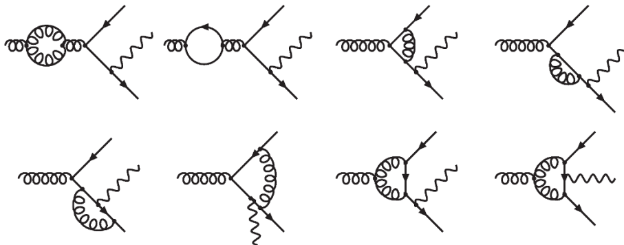
Figure 4. Representative diagrams contributing to the g \rightarrow q\bar{q}\gamma splitting amplitude.
