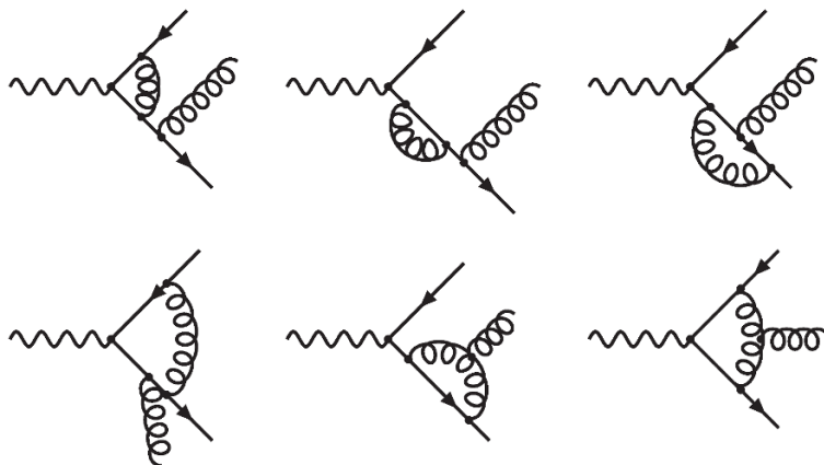
Figure 6. Representative diagrams contributing to the \gamma \rightarrow q\bar{q}g splitting amplitude.
