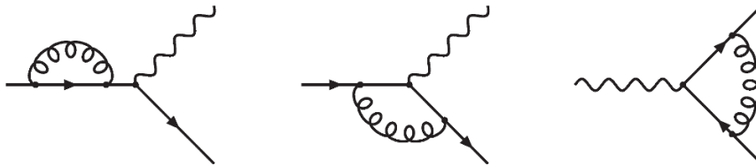
Figure 1. Feynman diagrams contributing to the splitting amplitudes of q \rightarrow q\gamma and \gamma \rightarrow q\bar{q} .
