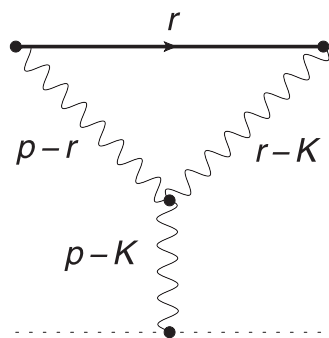
Figure 7. The non-Gaussian term in \mathcal{I} from I_B^{(2)} in equation (106).
