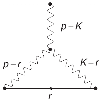
Figure 6. The non-Gaussian term in \mathcal{I} from I_B^{(1)} in equation (106).
