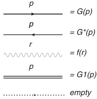
Figure 1. The graphic code we shall use in this paper. We represent G by a right pointing arrow, G^* by a left pointing one, f by a wavy line and G_1 by a double arrow. Points indicate that no propagator is assigned to that line.
