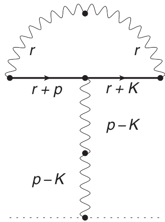
Figure 5. The term in \mathcal{I} from I_A^{(2)} in equation (106).
