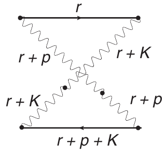
Figure 8. The term in \mathcal{I} from the maximally crossed graph I_A^{(3)} in equation (106). Observe that \mathbf{K} and \mathbf{p} appear as \mathbf{K} + \mathbf{p} ; no other graph has this feature at this order in the loop expansion.
