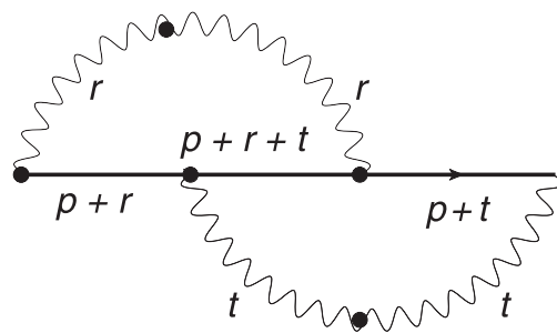
Figure 11. The two-loops contribution to the self-energy from Gaussian correlations.
