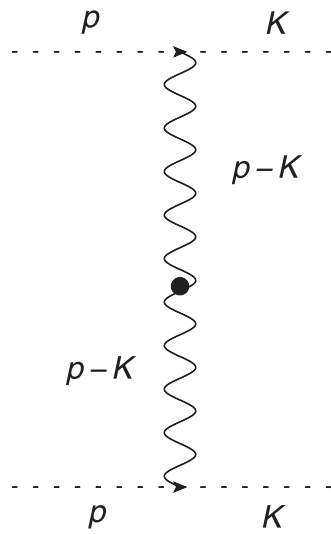
Figure 3. The term in \mathcal{I} from the ladder approximation.
