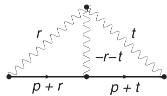
Figure 10. The two-loops contribution to the self-energy from non-Gaussian effects.
