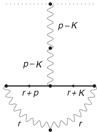
Figure 4. The term in \mathcal{I} from I_A^{(1)} in equation (106).
