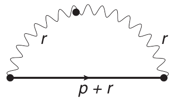
Figure 9. The one-loop contribution to the self-energy, which reproduces the so-called nonlinear approximation.
