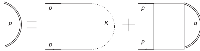
Figure 2. The Bethe-Salpeter equation (125) in graphic representation. A factor of \phi_0^2 is implicit in the first term in the right-hand side.
