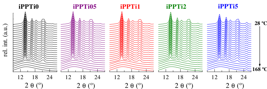
Fig. 5. Real-time variable-temperature WAXS profiles obtained with synchrotron radiation for all the quenched samples as processed in a melting experiment at 8 °C/min. Only one every three frames is plotted for clarity.
