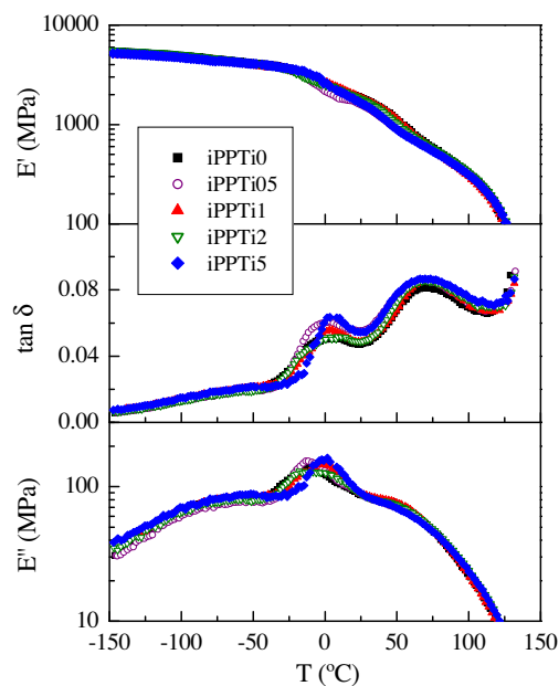
Fig. 11. Temperature dependence of the two components to the complex modulus ( E' and E'' ) and of the loss tangent ( \tan \delta ) for the neat homopolymer and its nanocomposites with distinct TiO 2 nanoparticle contents.
