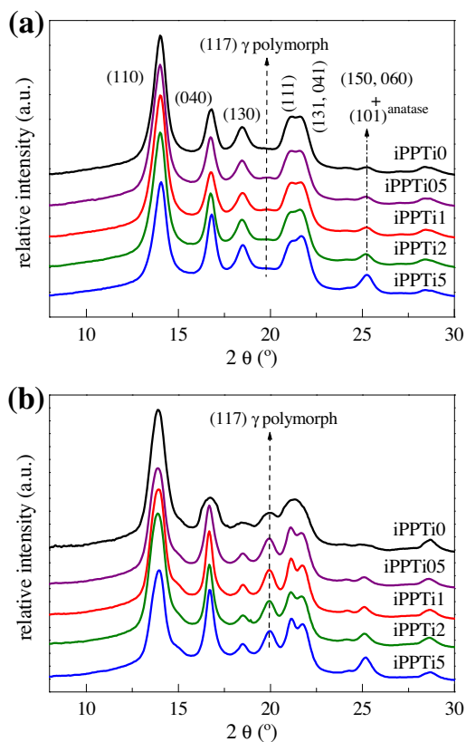
Fig. 4. WAXS diffraction patterns of pure iPP and the different nanocomposites at room temperature: (a) quenched films as processed and (b) samples crystallized at 8^\circ\text{C}/\text{min} after their first heating.
