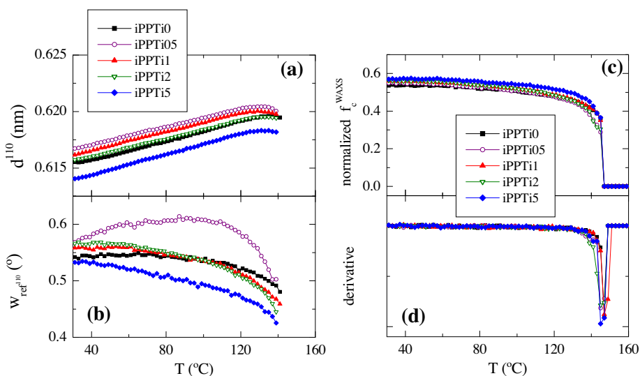
Fig. 6. Temperature dependence, on melting, for the (110) monoclinic reflection of: (a) peak spacing; (b) the width at half height of this diffraction; (c) normalized crystallinity determined from it; and (d) crystallinity derivative corresponding to the neat homopolymer and its nanocomposites.
