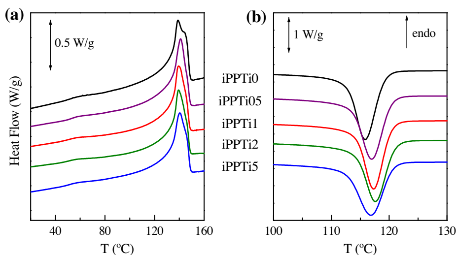
Fig. 9. DSC curves corresponding to: (a) the first heating process and (b) the crystallization corresponding to the neat homopolymer and its nanocomposites with distinct TiO 2 nanoparticle contents.
