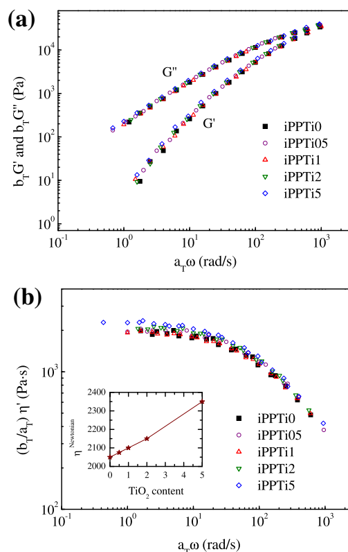
Fig. 2. (a) Reduced frequency dependence of storage modulus, G'(\omega) and loss modulus, G''(\omega) and (b) of dynamic viscosity ((b_T/a_T) \eta') observed in the metallocene iPP and its nanocomposites with TiO 2 .
