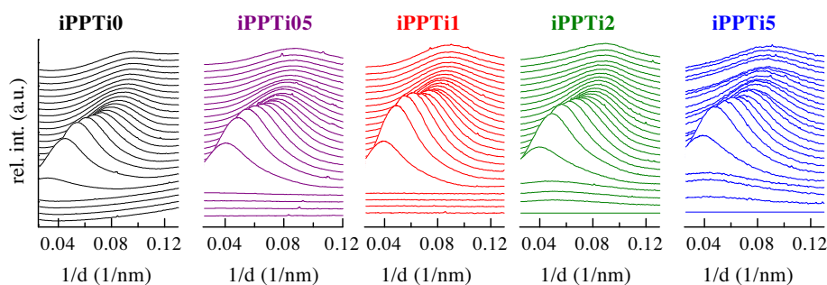
Fig. 7. Real-time variable-temperature Lorentz-corrected SAXS profiles obtained with synchrotron radiation for all the quenched samples as processed in a melting experiment from 28 to 168 °C at 8 °C/min. Only one every three frames is plotted for clarity.
