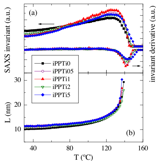
Fig. 8. Temperature dependence, on melting, of (a) the SAXS relative invariant and its derivative and (b) most probable long spacing corresponding to the neat homopolymer and its nanocomposites.
