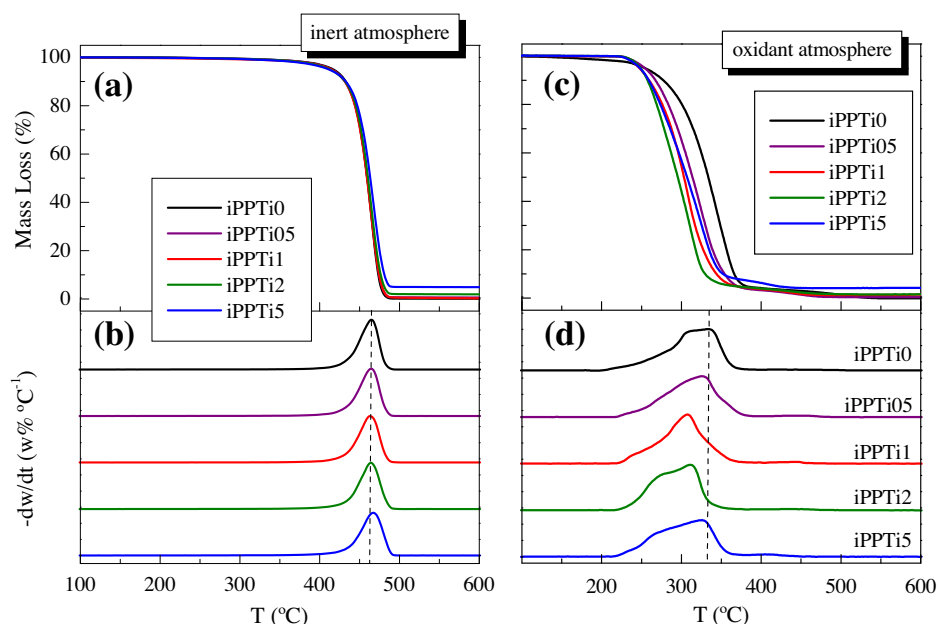
Fig. 10. Left plot: (a) TG and (b) DTG curves obtained under an inert atmosphere; Right plot: (c) TG and (d) DTG curves obtained under an oxidant atmosphere of neat homopolymer and the different nanocomposites analyzed. DTG curves have been vertically shifted for clarity.
