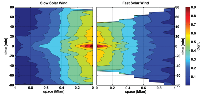
FIG. 3. Space-time correlation function R(|\mathbf{r}|, \tau) as function of magnitude of separation |\mathbf{r}| and \tau , for samples of (left) slow wind and (right) fast wind. Note that the orientation of axes differs from Fig 2. The time axis is vertical, and to facilitate the fast or slow wind comparison, space separation increases towards the left (right) for the slow (fast) wind case.
