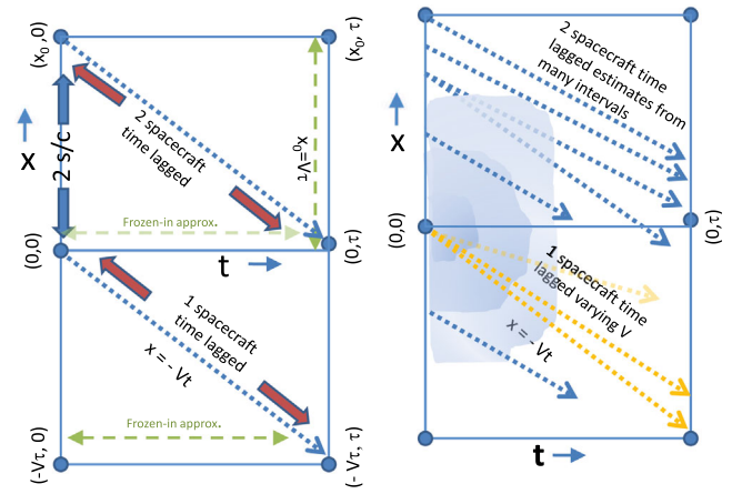
FIG. 1. (left) Space-time separation plane in the average solar wind plasma frame. Downward diagonal through the origin is the path observed by a single spacecraft (s/c). Vertical axis is the locus of pure spatial correlations. Taylor hypothesis approximates spatial correlation with single s/c correlation. The upper diagonal is the path observed by 2 s/c time-lagged correlations. (right) With many samples, it is feasible to obtain substantial information about the plasma frame space-time correlation. Here only one spatial coordinate is shown for simplicity.
