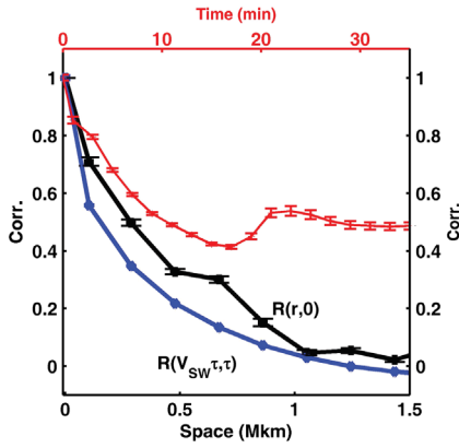
FIG. 4. Correlation function R(|\mathbf{r}|, \tau) sampled along three directions in space-time. (black, squares) Purely spatial correlation R(r, 0) plotted vs r ; (blue, diamonds) Typical observation made in a solar wind flow at speed V_{sw} by a single spacecraft, R(V_{sw}\tau, \tau) . These are approximated as equal in the Taylor hypothesis. Third curve (red, plus signs) is the purely temporal correlation R(0, \tau) plotted vs \tau on the upper axis. Error bars (standard error of the mean) are representative of counting statistics throughout the analysis.
