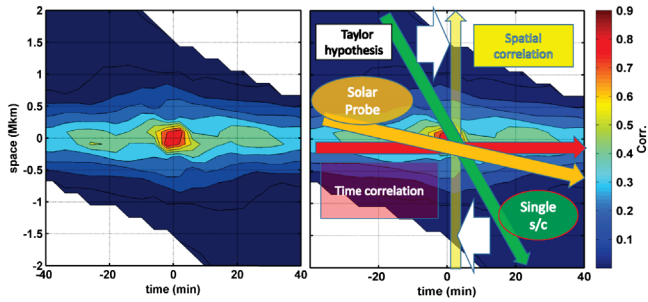
FIG. 2. (left) Space-time correlation of the full ensemble of solar wind magnetic field interval pairs described in the text, presented in the format R(r, *, *, \tau) , where the “*” indicate averaging over the transverse separations. (right) Same correlation, with annotations showing various sampling directions: spatial correlation, time correlation, fast single spacecraft trajectory, and slow spacecraft trajectory, such as Solar Probe. The content of the Taylor hypothesis is illustrated, as described in the text.
