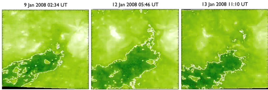
Figure 4 Three individual SOHO/EUV Imaging Telescope (EIT) 195 Å image frames from a movie covering the interval 9 to 13 January which illustrates the boundary evolution of CH2. Although viewing angles do influence the CH boundaries, the dynamic nature of the CH boundary is evident. The images represent a 700'' \times 700'' area. See the corresponding movies in the electronic supplement to this article in the electronic version both with and without the contours indicating the boundary of the CH.
