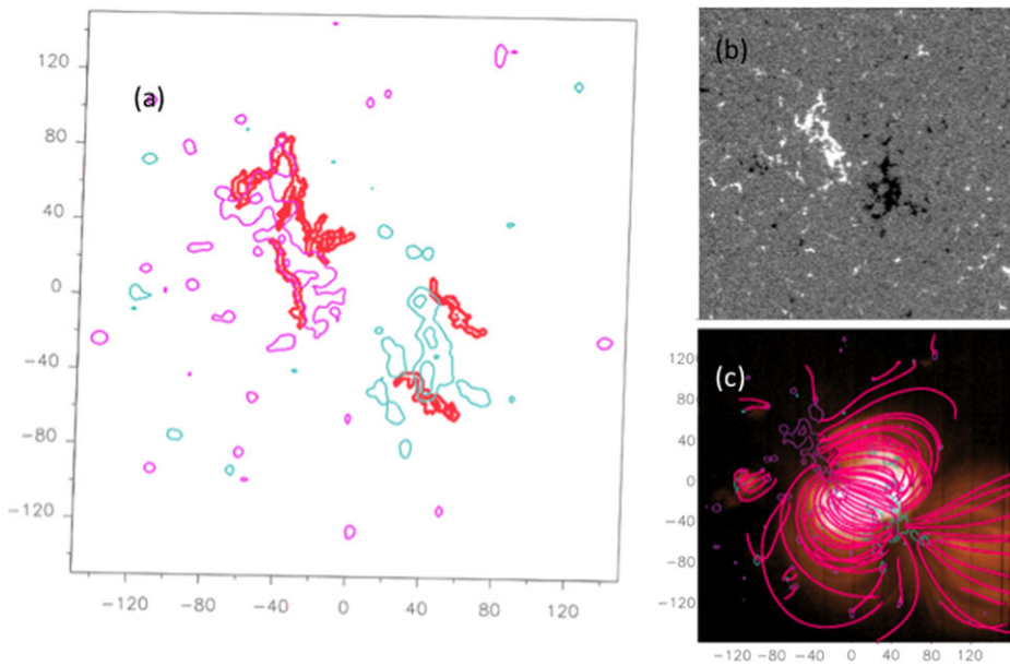
Figure 6 (a) Photospheric trace of dominant QSLs indicated by the thick red lines overlaid on an MDI magnetogram (turquoise/magenta is negative/positive, -50/50 G and -300/300 G contours). The most extended QSL trace is located over the positive polarity of the AR within the EIS FoV. For context, (b) an MDI magnetogram, and (c) an Fe XV image overlaid with field lines from the same LFFF model used for computing the QSLs in panel (a) for AR2 are shown on 10 January 2008.
