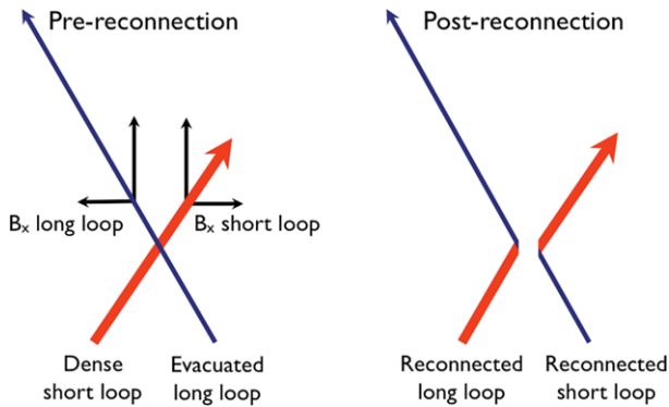
Figure 5 Simplified 2D cartoon explanation of magnetic reconnection between two positive-polarity magnetic loops (field lines) having a non-zero angle between them. This type of magnetic component reconnection can take place along QSLs at the periphery of an AR, e.g. between dense loops of the AR and more evacuated loops connecting elsewhere outside or inside the AR. (Left) Pre-reconnection configuration: the dense closed AR-loop field line (thick red line) and the evacuated far-closing field line (thin blue line) have an anti-parallel B_x component. Along the QSL between these field lines of drastically different connectivities, a current sheet forms enabling reconnection. (Right) These field lines “break” and reconnect. The far-connecting post-reconnection field line shown on the left will have a dense lower and an evacuated upper part, while the reconnected short field line has densities the other way around. The resulting density gradients drive plasma flows upward along the long field line, leading to blue-shifted plasma flows and downward along the short field line (AR-loop), leading to red-shifted flows.
