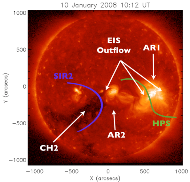
Figure 12 Hinode /XRT image on 10 January 2008. Both active regions (AR1, AR2), the second coronal hole (CH2), and stream interaction region (SIR2) are indicated. Also shown are the positions of the active-region outflow sites observed with Hinode /EIS and the Heliospheric Plasma Sheet (HPS) location projected radially on the Sun.
