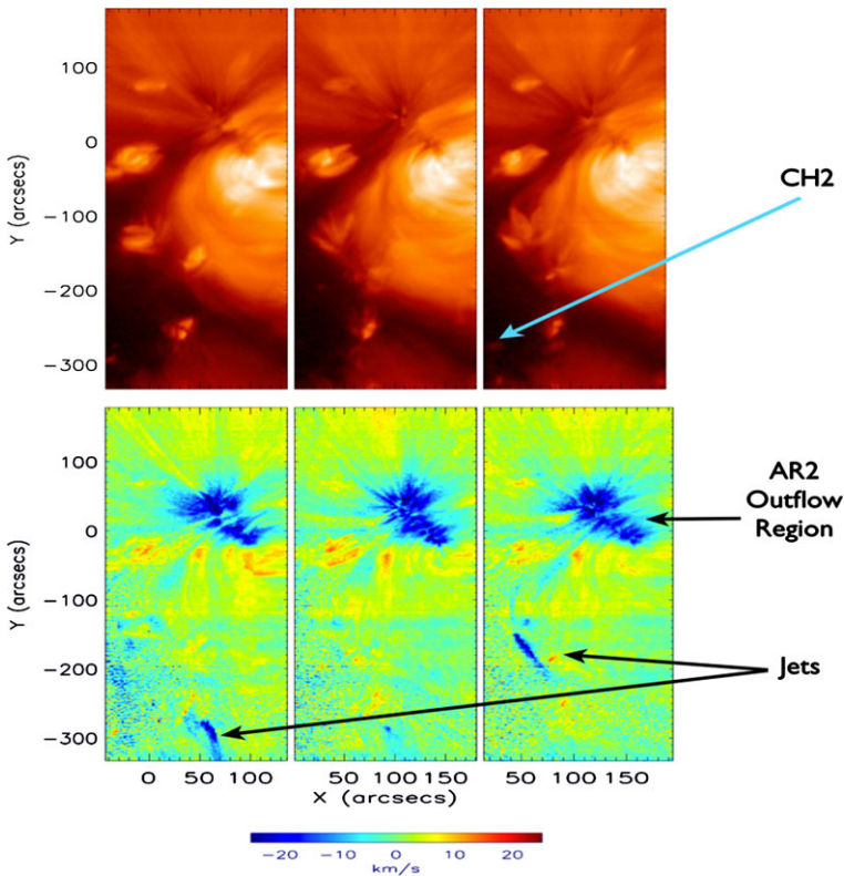
Figure 3 Set of three EIS Fe XII ( T_e \approx 10^{6.1} K) intensity maps (top row) and the corresponding velocity maps (bottom row). Reading left to right, maps were obtained on 10 January 2008 at 18:08 UT and at 22:51 UT and on 11 January 2008 at 00:17 UT. CH2 is indicated in the upper panel while the strong and variable outflow region at the NE edge of AR2 is shown in the velocity maps, as are two coronal jets.
