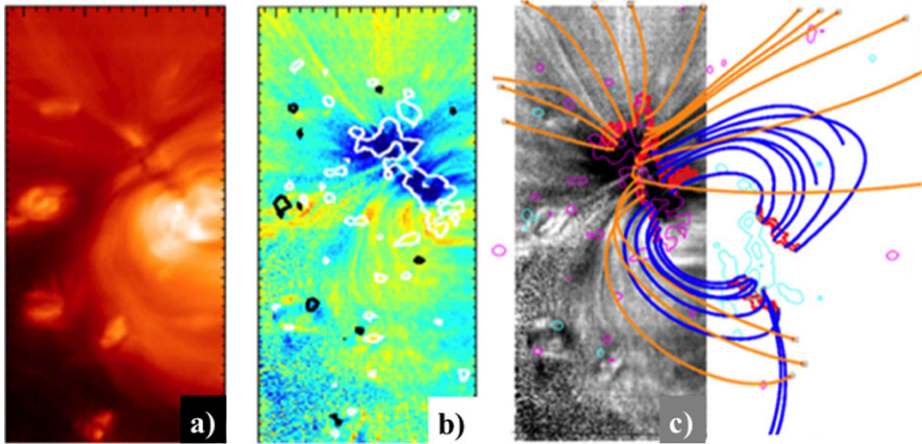
Figure 7 (a) EIS Fe XII intensity map of AR2. (b) Fe XII velocity map overlaid with \pm 50 G MDI magnetic contours. White/black is positive/negative polarity. (c) Photospheric trace of QSLs (thick red lines) and field lines originating in the QSLs computed from a LFFF extrapolation. They are overlaid on a greyscale polarity map. Orange/blue field lines are drawn from the QSL over the positive polarity. Lines with circles leave the viewing 3D box and are considered to be open or large extended loops. Magnetic field isocontours are shown in continuous magenta/turquoise lines for positive/negative values of the field ( \pm 50 G and \pm 300 G).
