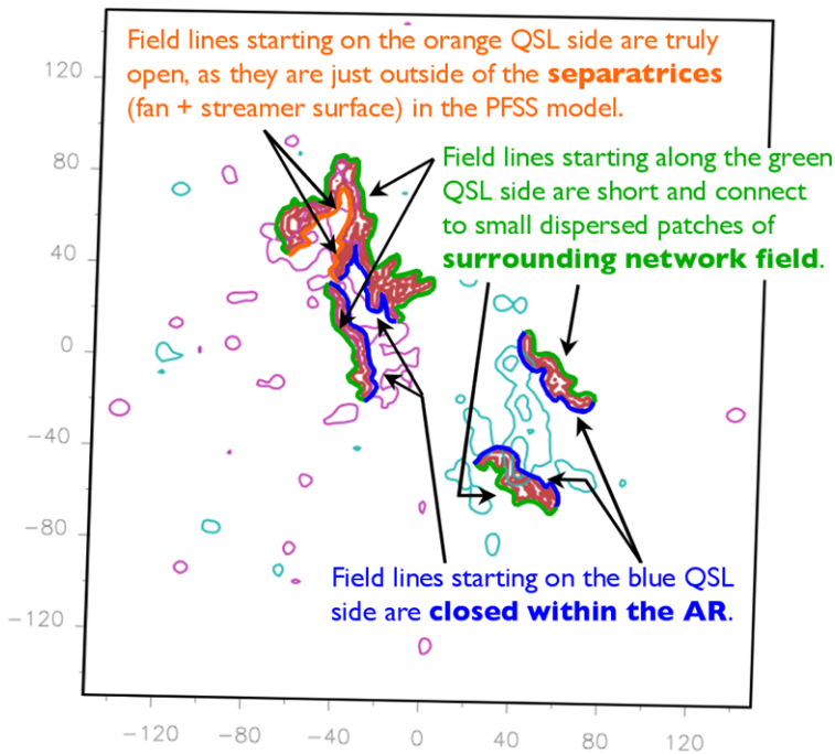
Figure 11 QSL locations in AR2 ( cf. Figure 6 where QSLs are shown in dark red) with the types of connectivity on both sides colour-coded and the characteristic connectivities described using the insight gained from PFSS modeling. The QSLs are overlaid on an MDI magnetogram where isocontours of the polarities are represented with different colours (turquoise is negative, magenta is positive polarity). Different sides of each QSL are coloured according to the field line connectivity found.
