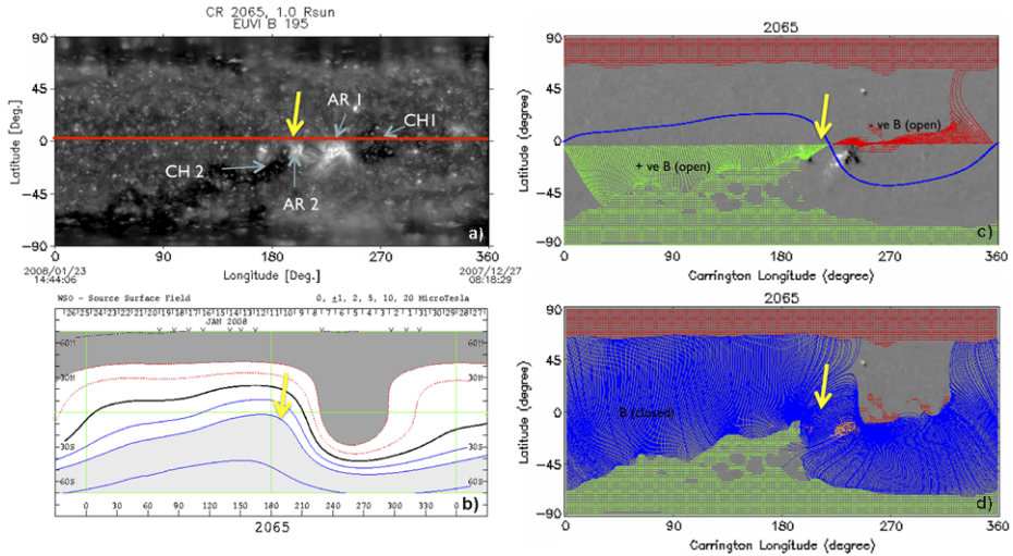
Figure 2 (a) Carrington Rotation 2065 displayed with STEREO-B/EUVI images. (b) Wilcox Solar Observatory PFSS model for CR 2065 with isocontours of the large-scale radial field component. Grey areas show the open-field regions. (c) NSO/GONG PFSS model with open field reaching the ecliptic plane (shown up to the source surface at 2.5 R_{\text{Sun}} ). The AR and CH features shown in Figure 1 are indicated, while the solar Equator is drawn in red. The red/green areas show the negative/positive polarity of the open-field regions and the blue line is the inversion line at 2.5 R_{\text{Sun}} . (d) As for (c) but showing the largest closed field lines (reaching 2.5 R_{\text{Sun}} ). The yellow arrow indicates the studied site of the EIS outflow from AR2.
