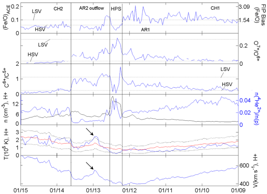
Figure 13 ACE in-situ observations of SW plasma for the interval 9–15 January 2008 (right to left). From the top of the figure, values of the concentration ratios Fe/O , O^{7+}/O^{6+} , C^{6+}/C^{5+} , and He^{2+}/H^+ , and density, temperature, and proton velocity are plotted against time. The FIP bias, i.e. Fe/O normalized to photospheric value, is indicated on the top right. In the three top panels the typical low- and high-speed values (LSV and HSV) are indicated by the horizontal dotted lines. The expected temperature in a SW with the same velocity is shown in red, while dotted lines show the typical extreme values in the T panel. Passage of the HPS is indicated as are those of CH2, AR2, AR1, and CH1. The black arrows show a proton-velocity and temperature peak, which we link to outflows from AR2.
