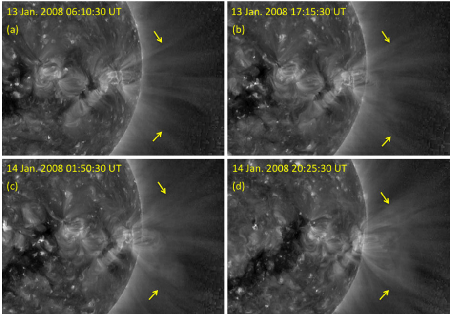
Figure 15 STEREO-A 195 Å EUVI images of the AR–CH complex showing loops fanning out of AR1. These loops become increasingly visible as AR1 approaches the limb. Although PFSS modeling indicates that AR1 is fully enveloped by the streamer above it, the dynamically changing loops fanning out of the AR1–CH1 interface indicate that the boundary is not simple and there is a continuous interchange reconnection process, taking place low in the corona driving brightness changes in the fan. The frames shown here have been wavelet-cleaned and enhanced to extend the visibility of the coronal features as far out as possible above the limb (see Stenborg, Vourlidas, and Howard, 2008, for a description of the method). See the corresponding movie in the electronic supplement to this article in the electronic version.
