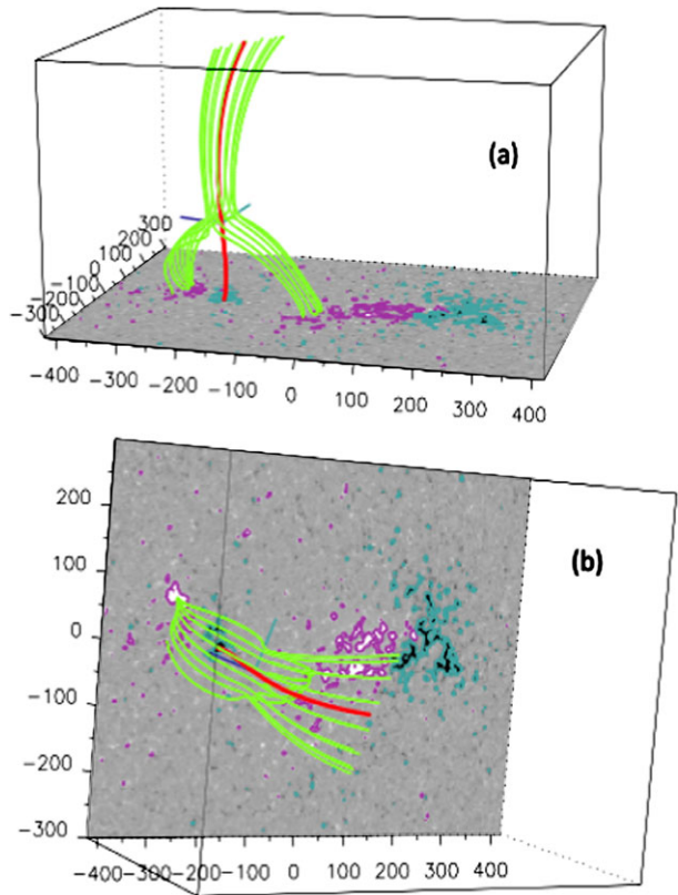
Figure 8 Location of a high-altitude (about 130 Mm) null point above AR2 in the AR1–AR2 complex in a Cartesian potential-field extrapolation. The spine field line (red) and fan field lines (green lines) are shown from two perspectives (a) from the South and (b) as seen from Earth. The bottom boundary is an MDI magnetogram taken on 9 January 2008, when the AR1–AR2 complex was closest to the central meridian. Negative polarity is contoured with turquoise, positive with magenta.
