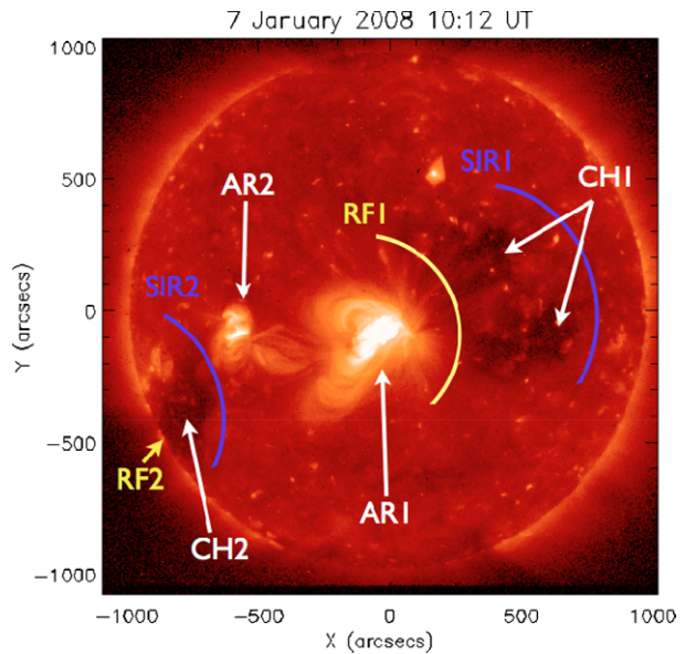
Figure 1 Hinode /XRT image for 7 January 2008. Markings show a stream interaction region (SIR1), a coronal hole (CH1), a rarefaction region (RF1), and two active regions (AR1 and AR2), followed by a second stream interaction region (SIR2), coronal hole (CH2), and rarefaction region (RF2). SIR1, RF1, and RF2 locations are shown projected radially on the Sun.
