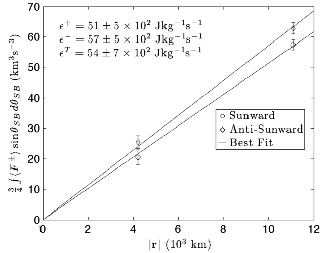
FIG. 2. Linear scaling of the (circles) sunward and (diamonds) antisunward components of the third-order law. The solid lines are least squares fits to the data that have the added restriction of passing through the origin. It is the gradients of these lines that correspond to the mean volume averaged cascade rates. The total energy transfer rate, which becomes the dissipation rate at small scales, is the average of the sunward and antisunward components.
