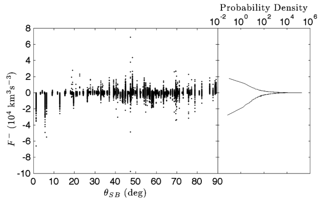
FIG. 1. All estimates of the antisunward normalized flux density with the corresponding PDF, both highlighting the almost symmetrical character of the mixed third-order statistic. There is good \theta_{SB} coverage, but it is nonuniform: sparser parallel and perpendicular to the mean magnetic field direction, \theta_{SB} = 0-10^\circ and \theta_{SB} = 80-90^\circ . The smoothness of the PDF, where each bin contains around 100 data points, implies that the associated statistical quantities are well defined.
