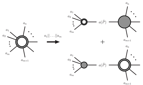
Figure 2. Factorization of one-loop amplitudes in the multiple collinear limit.
