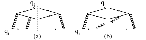
Figure 3. Example of (a) virtual and (b) real contributions to P_{ns}^{(2)S} .
