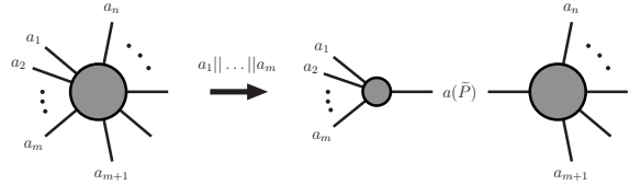
Figure 1. Factorization of tree-level amplitudes in the multiple collinear limit.
